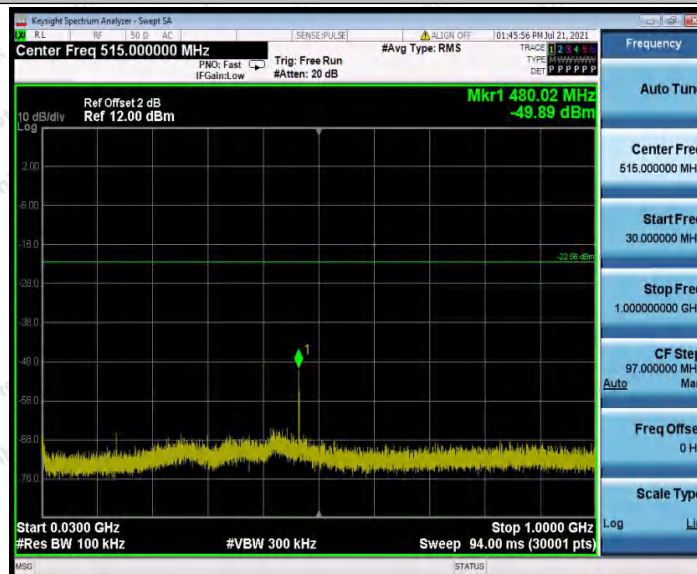
11N40_Ant2_2437_30~1000
