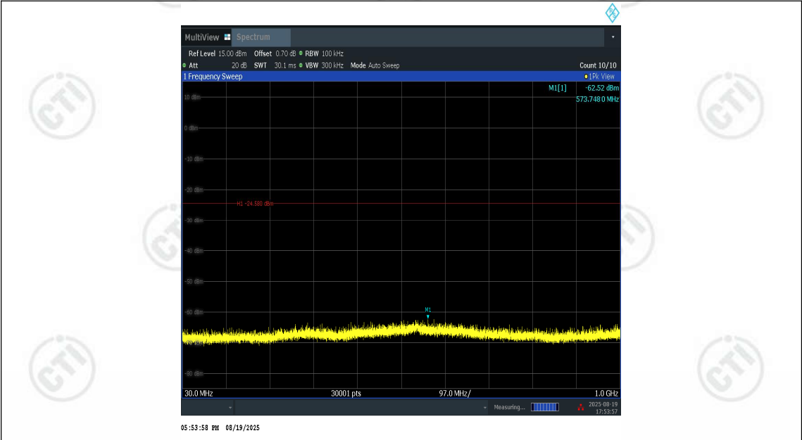
11N20SISO-Ant1-2437-30~1000-PASS
