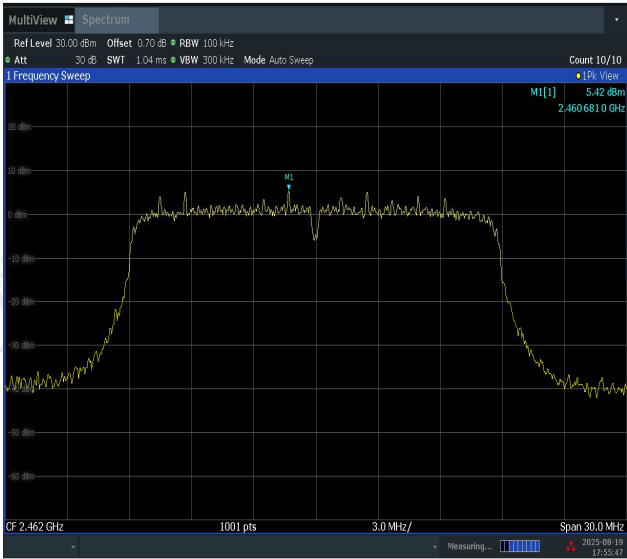
11N20SISO-Ant1-2462-0~Reference-PASS
