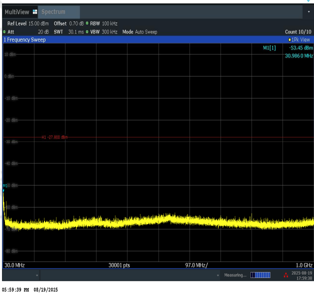
11N40SISO-Ant1-2437-30~1000-PASS
