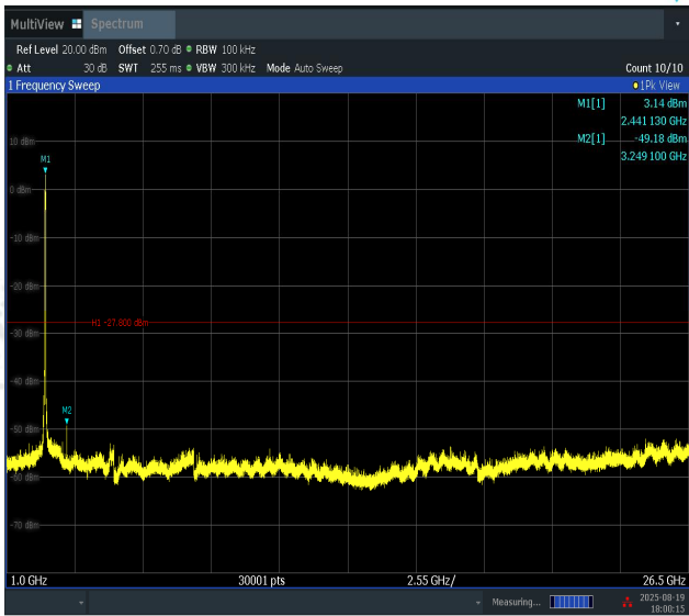
11N40SISO-Ant1-2437-1000~26500-PASS
