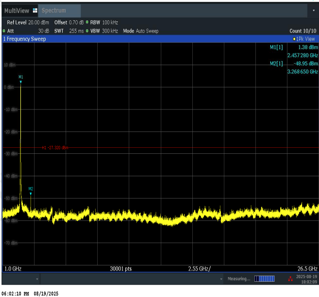
11N40SISO-Ant1-2452-1000~26500-PASS
