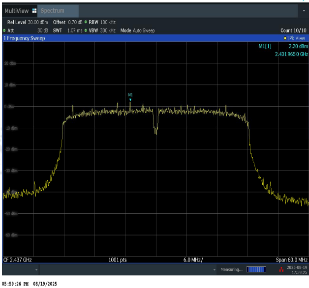
11N40SISO-Ant1-2437-0~Reference-PASS
