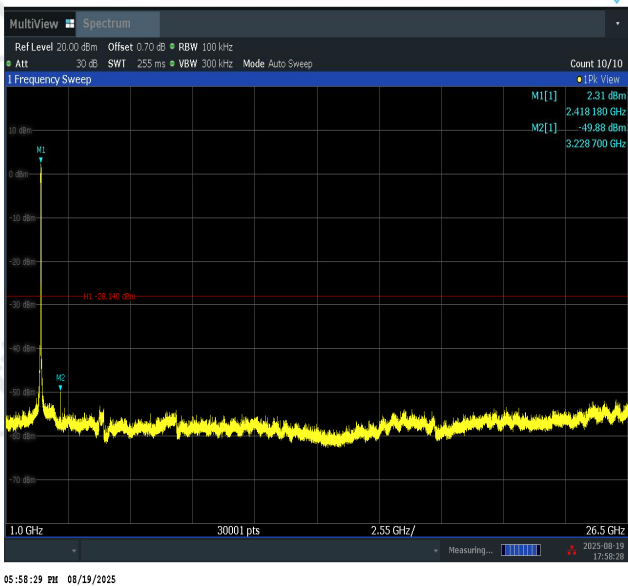
11N40SISO-Ant1-2422-1000~26500-PASS
