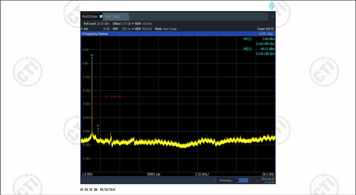
11N20SISO-Ant1-2437-1000~26500-PASS
