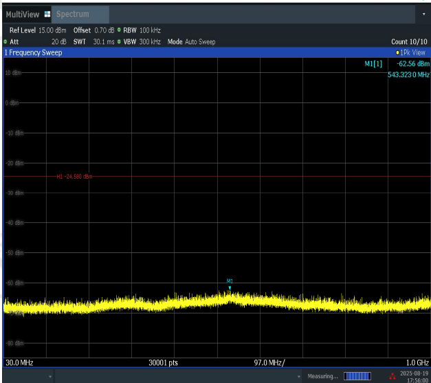
11N20SISO-Ant1-2462-30~1000-PASS
