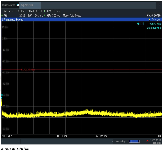
11N40SISO-Ant1-2452-30~1000-PASS
