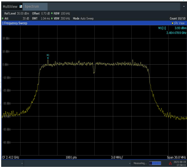
11N20SISO-Ant1-2412-0~Reference-PASS
