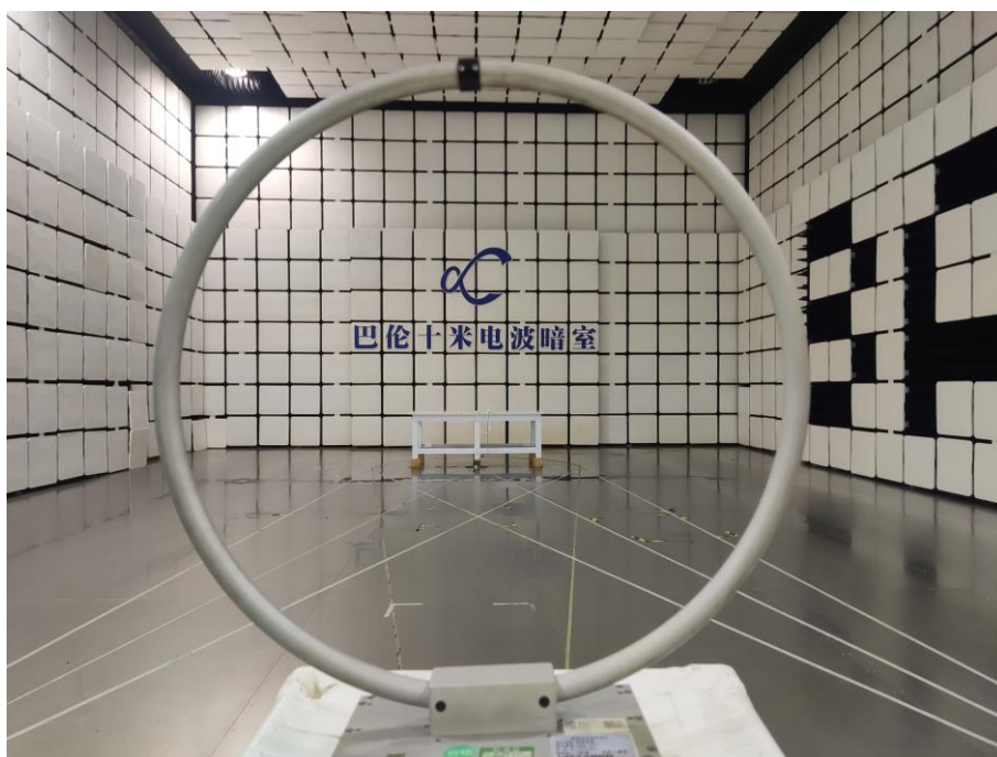
Below 30MHz-LoRa
