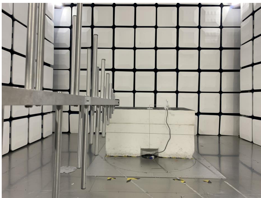
30MHz-1GHz-LoRa
