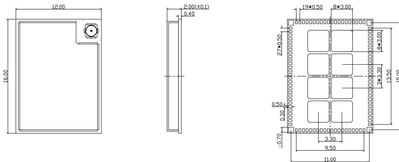
Figure 5-1-2. BM3301-1216 Module Package Outline Drawing
