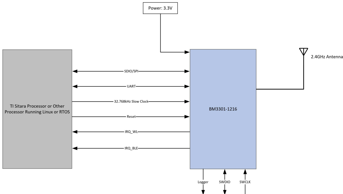
Figure 5-3-1. System Block Diagram
