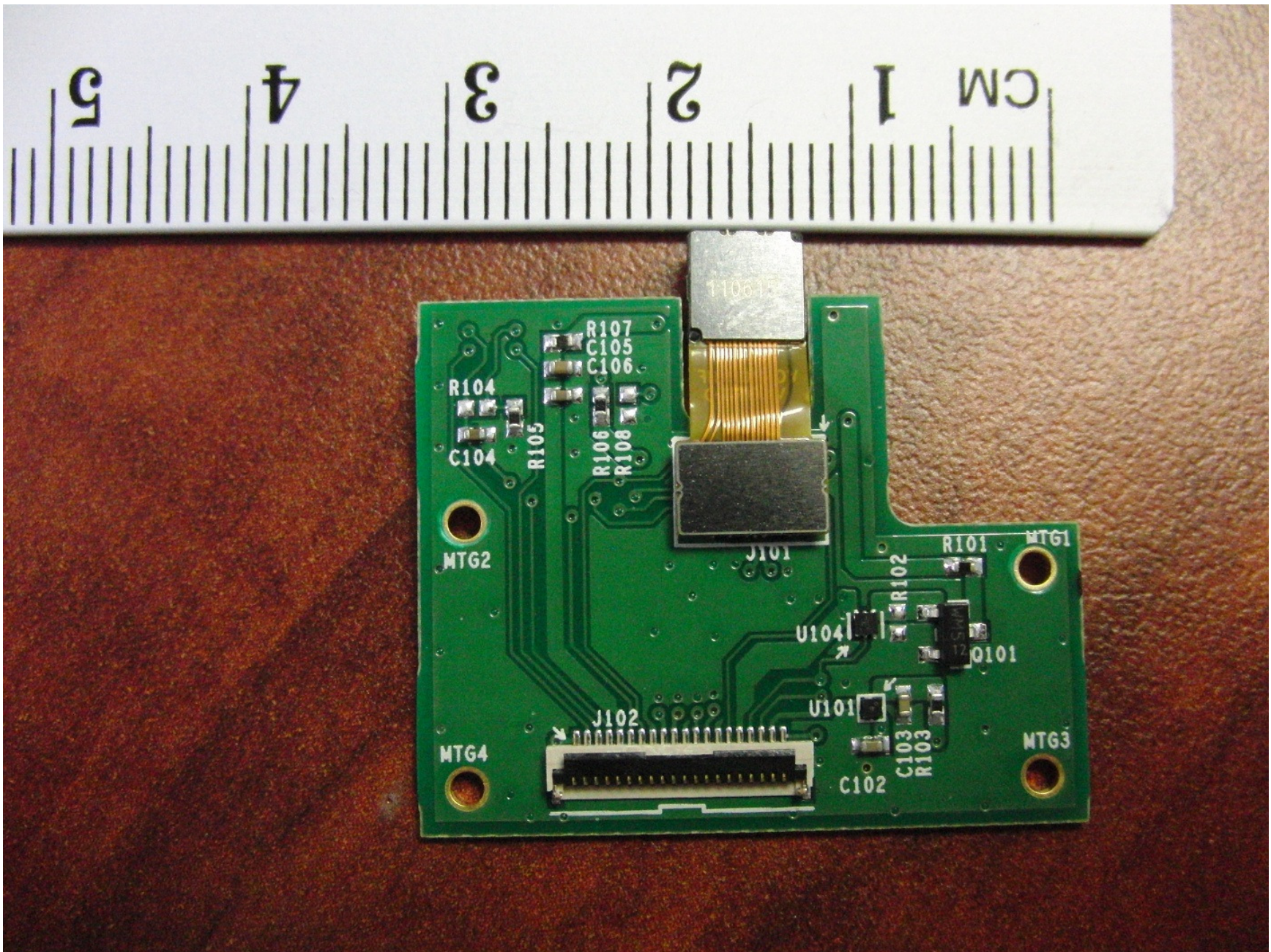
Photo 2: MS009 PCB Assembly, Bottom View
