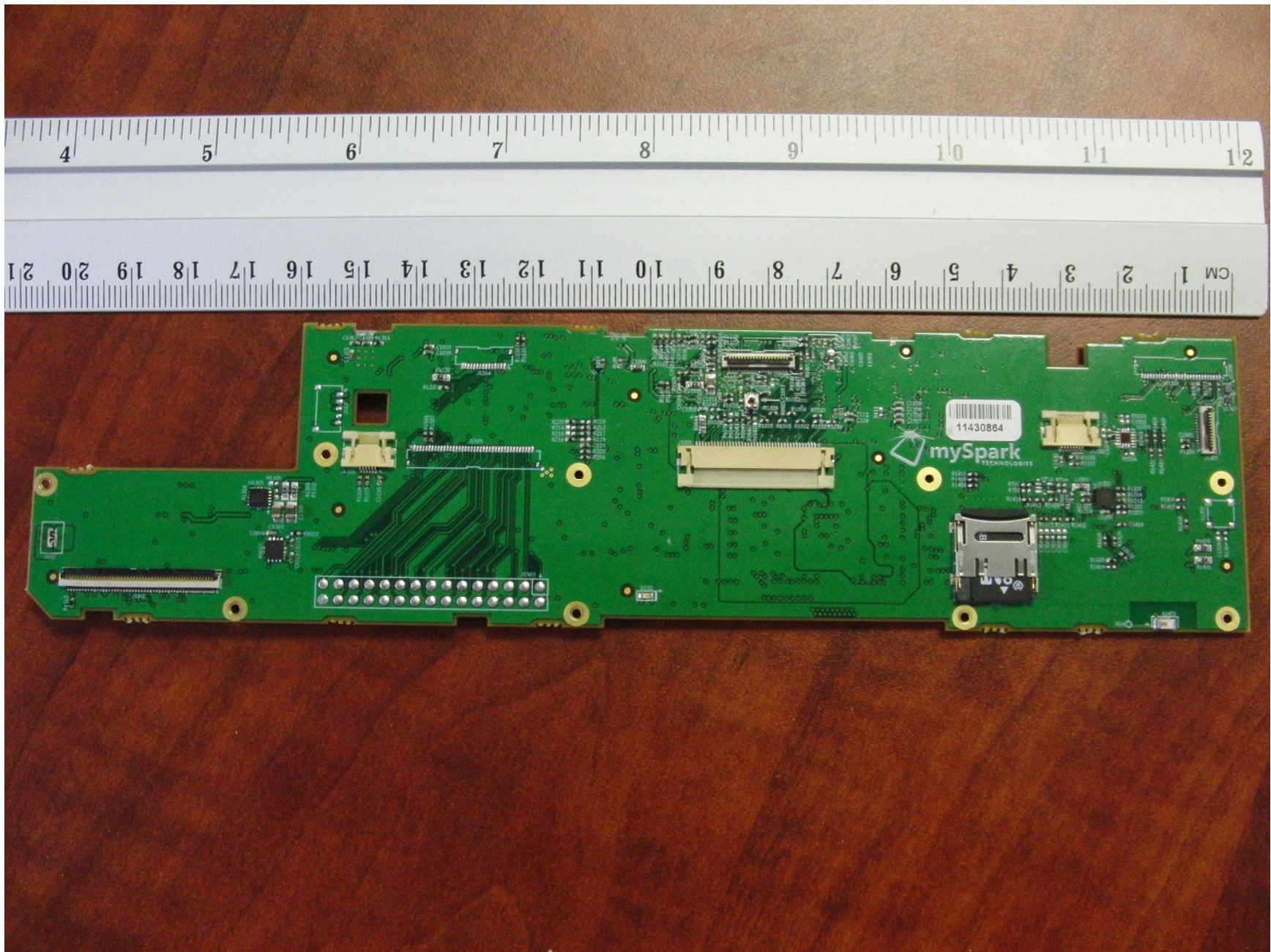
Photo 6: MS006 PCB Assembly, Bottom View
