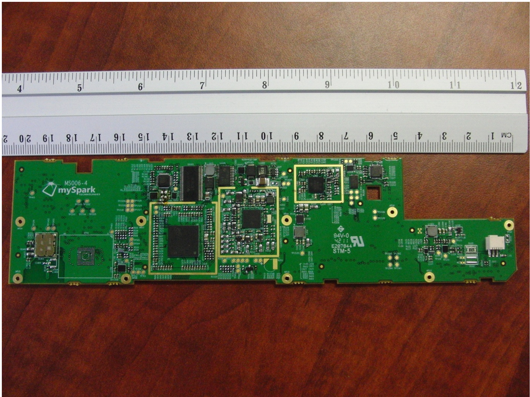
Photo 7: MS006 PCB Assembly, Top View
