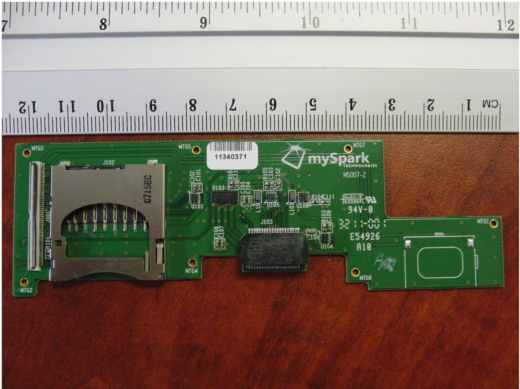
Photo 5: MS007 PCB Assembly, Top View
