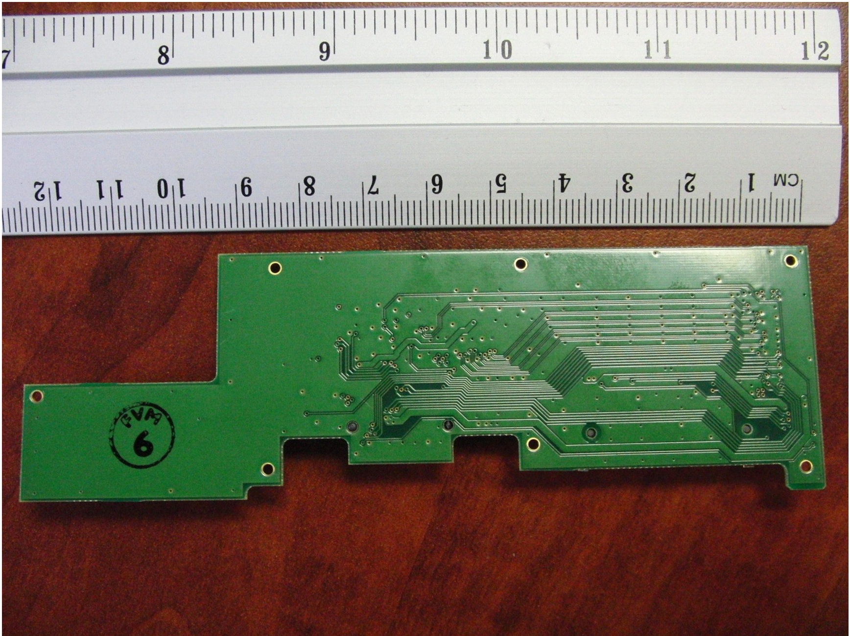
Photo 4: MS007 PCB Assembly, Bottom View
