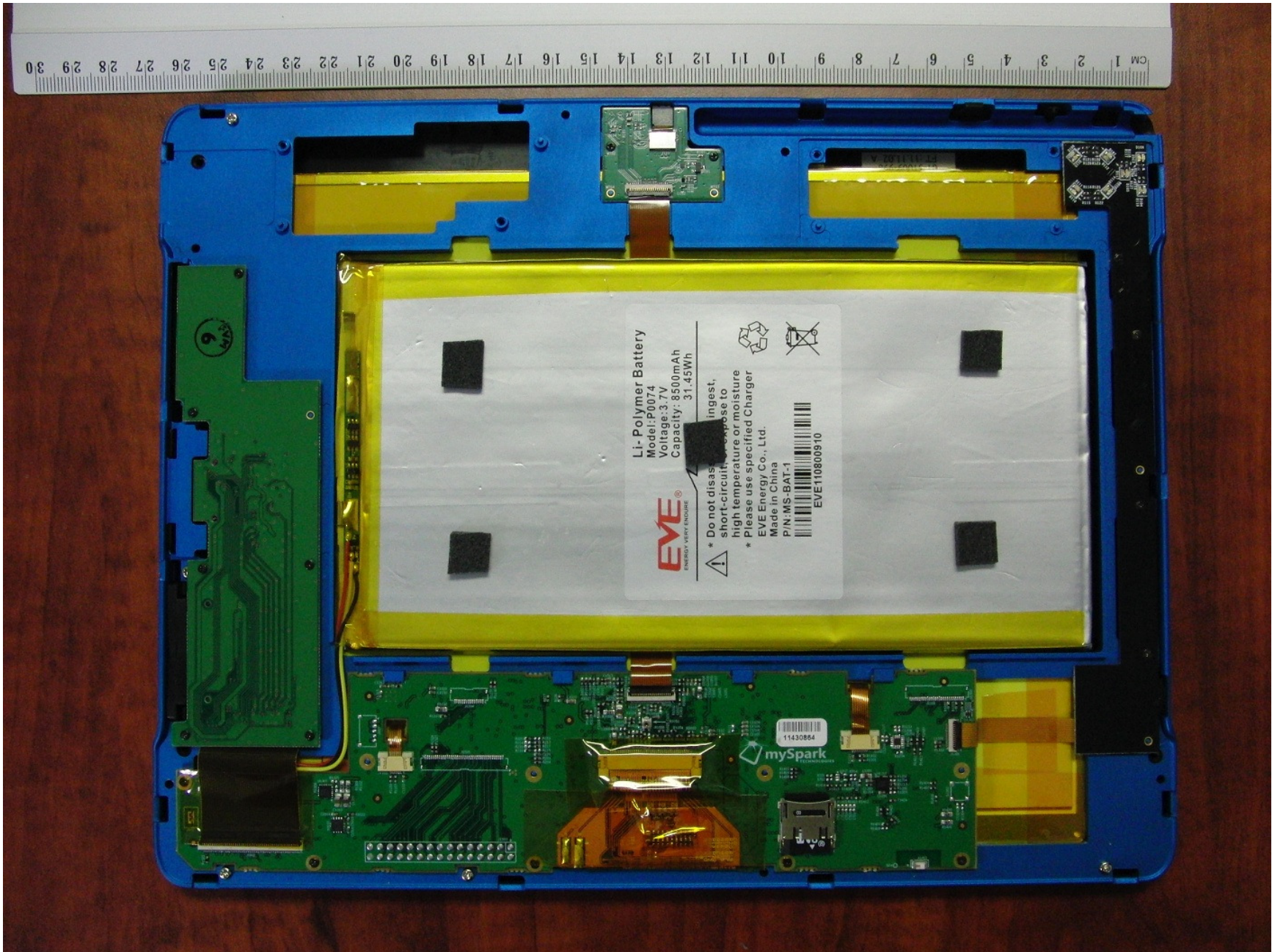
Photo 1: Internal View
