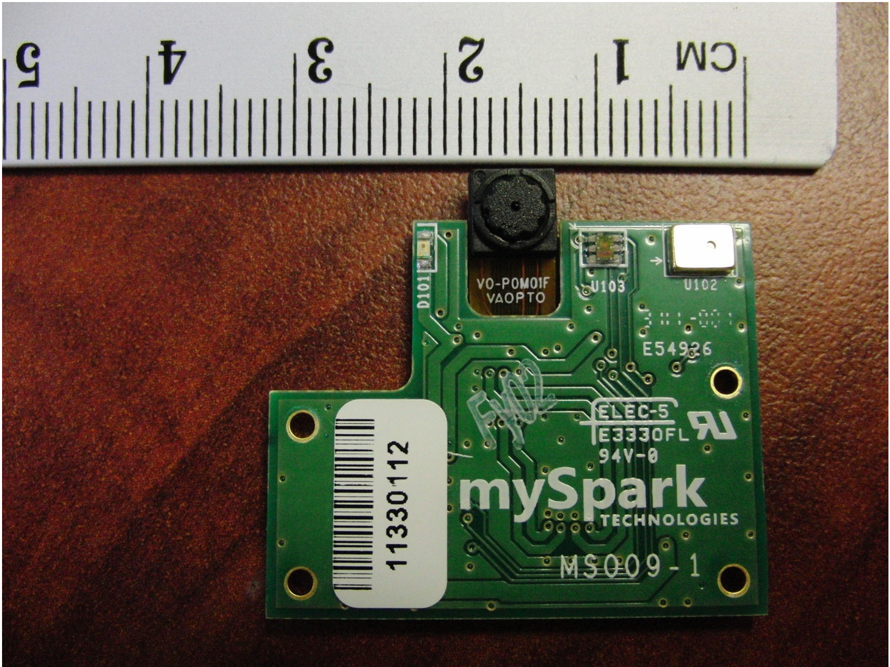
Photo 3: MS009 PCB Assembly, Top View
