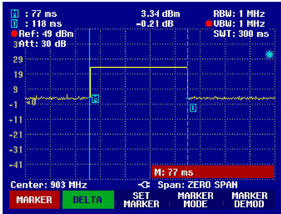
Graph 9 Average Time of occupancy of hopping frequency
