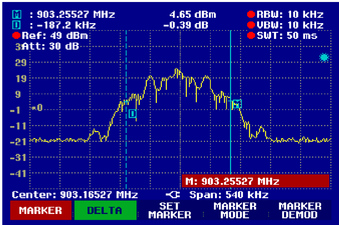
Graph 5 20dB bandwidth (low frequency channel)
