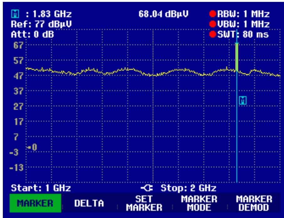
Graph 18 Radiated Spurious Emissions 1 GHz – 2 GHz Vertical and Horizontal
