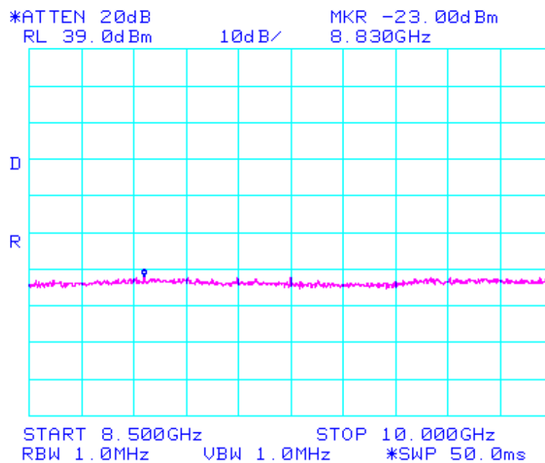
Graph 17 Conducted Spurious Emissions 8.5-10 GHz
