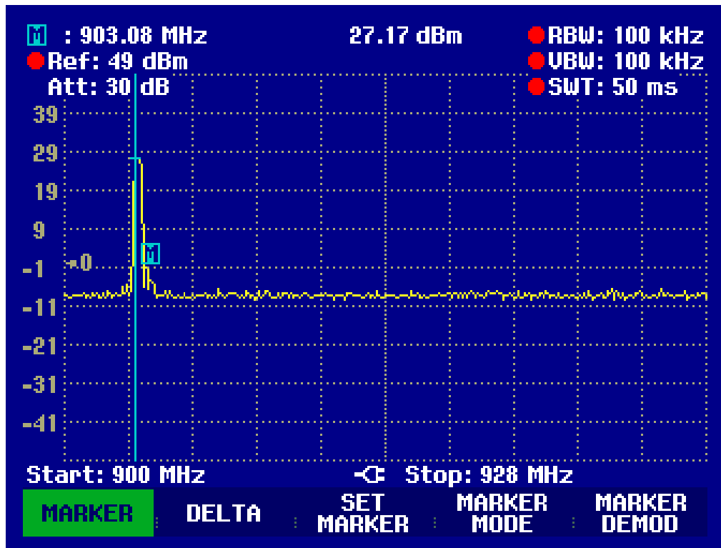
Graph 11 (lower frequency channel)
