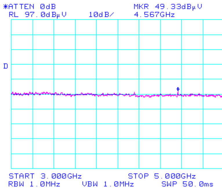
Graph 18 Radiated Spurious Emissions 3 GHz – 5 GHz Vertical and Horizontal
