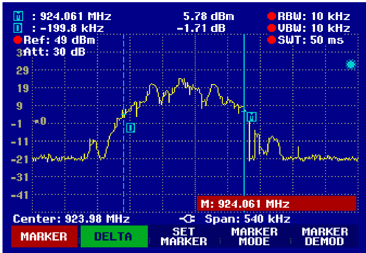
Graph 7 20dB bandwidth (upper frequency channel)
