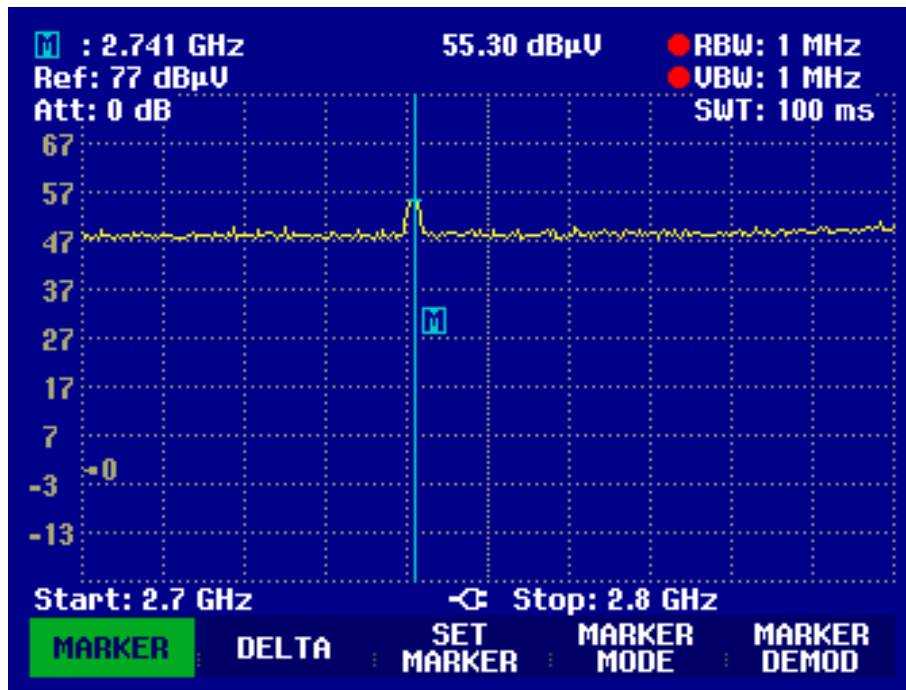
Graph 18 Radiated Spurious Emissions 2.7 GHz – 2.8 GHz Vertical and Horizontal
