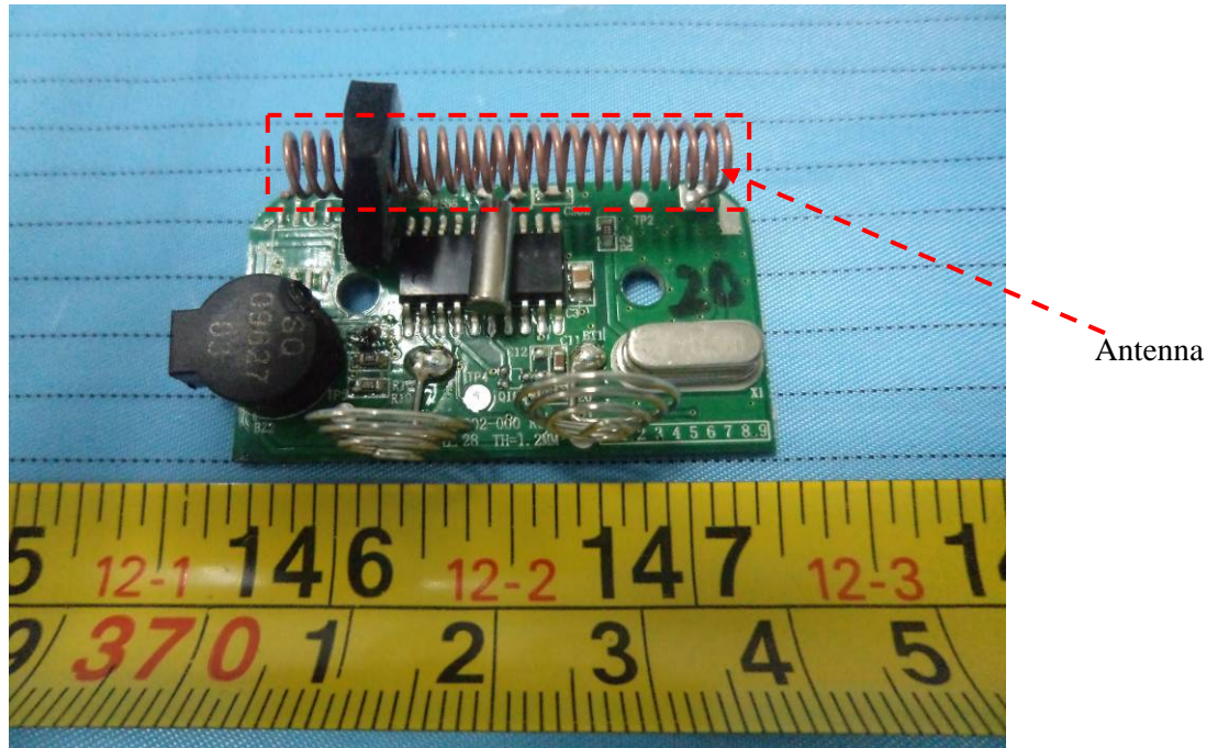
EUT- Mainboard Components View
