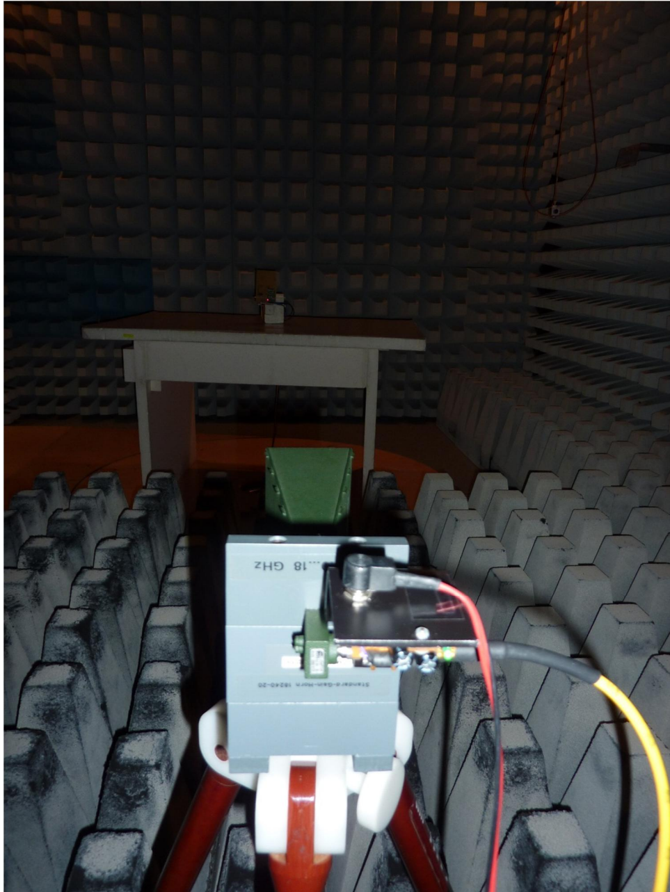
113483_4: Test setup fully anechoic chamber
