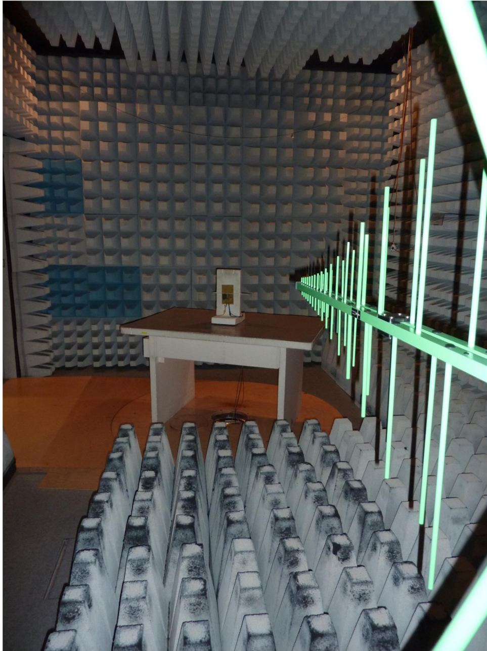
113483_2: Test setup fully anechoic chamber
