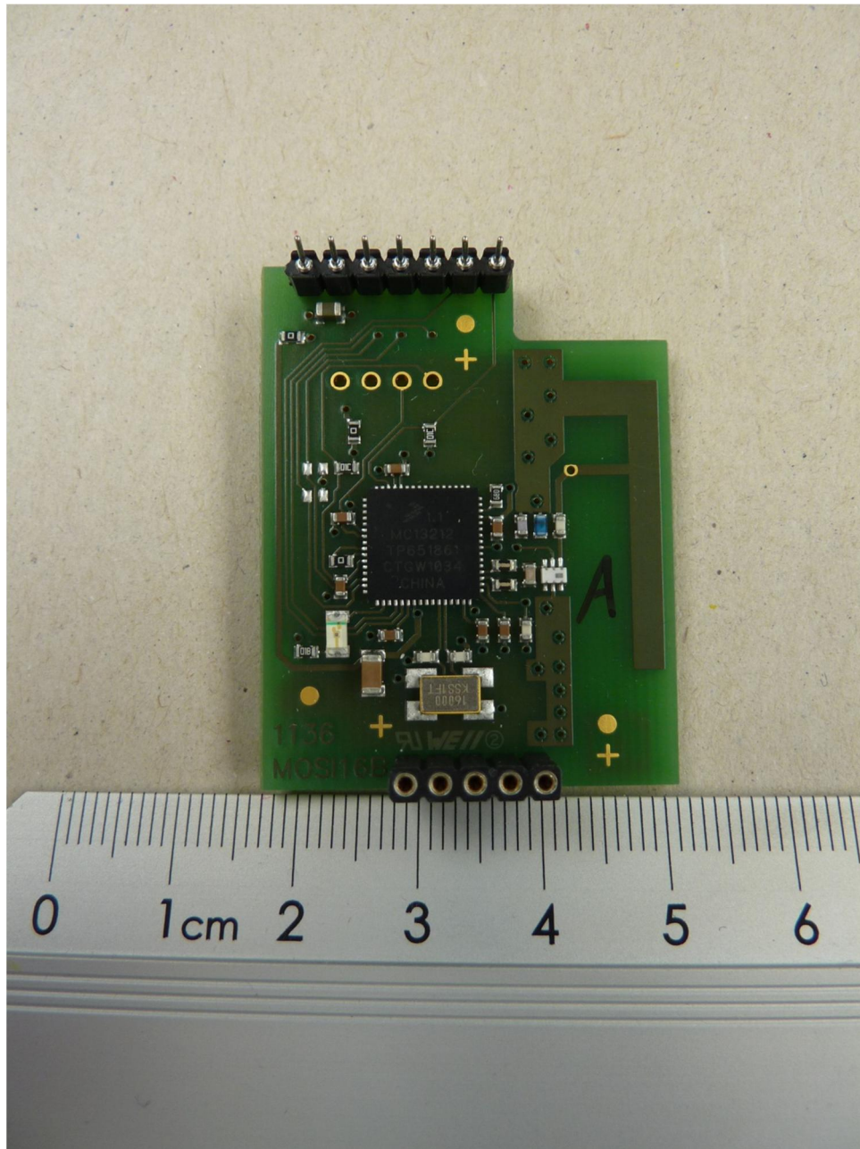
113483_9: MOSI16B, top view
