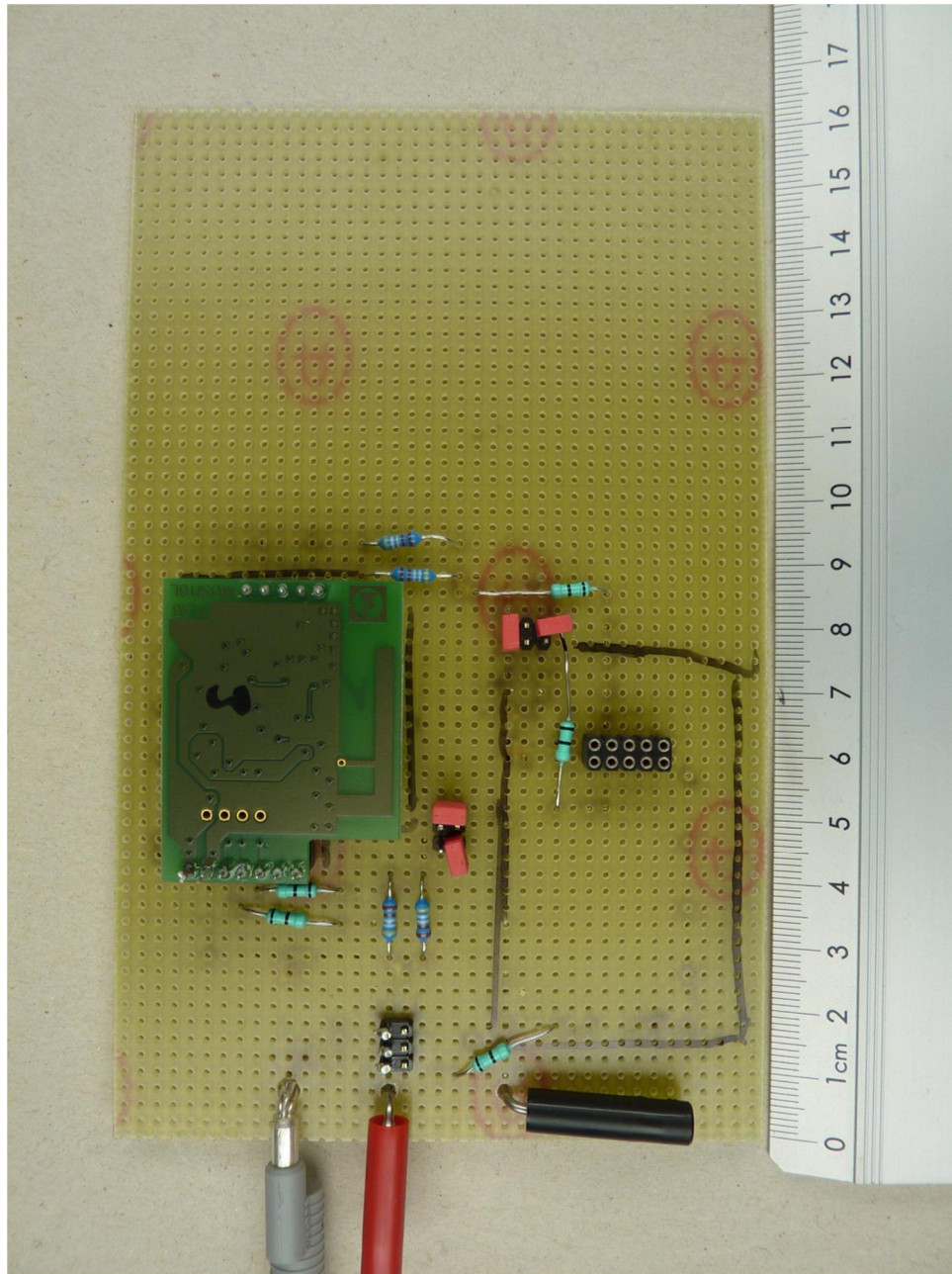
113483_7: MOSI16B mounted on carrier board, top view
