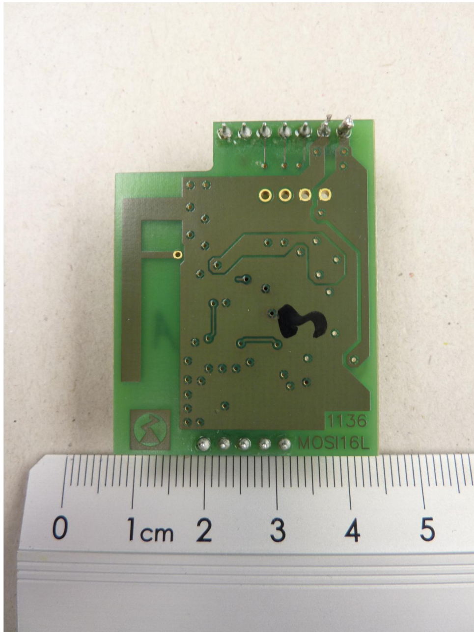
113483_10: MOSI16B, bottom view
