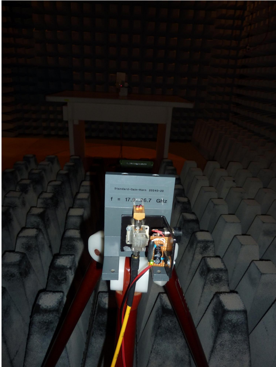
113482_11: Test setup fully anechoic chamber
