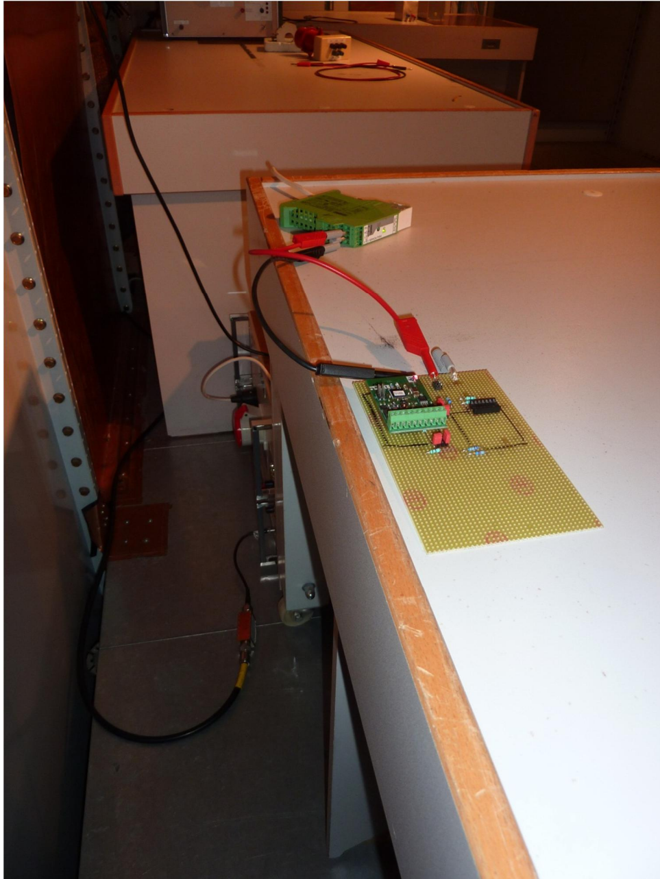
113482_13: Test setup shielded chamber
