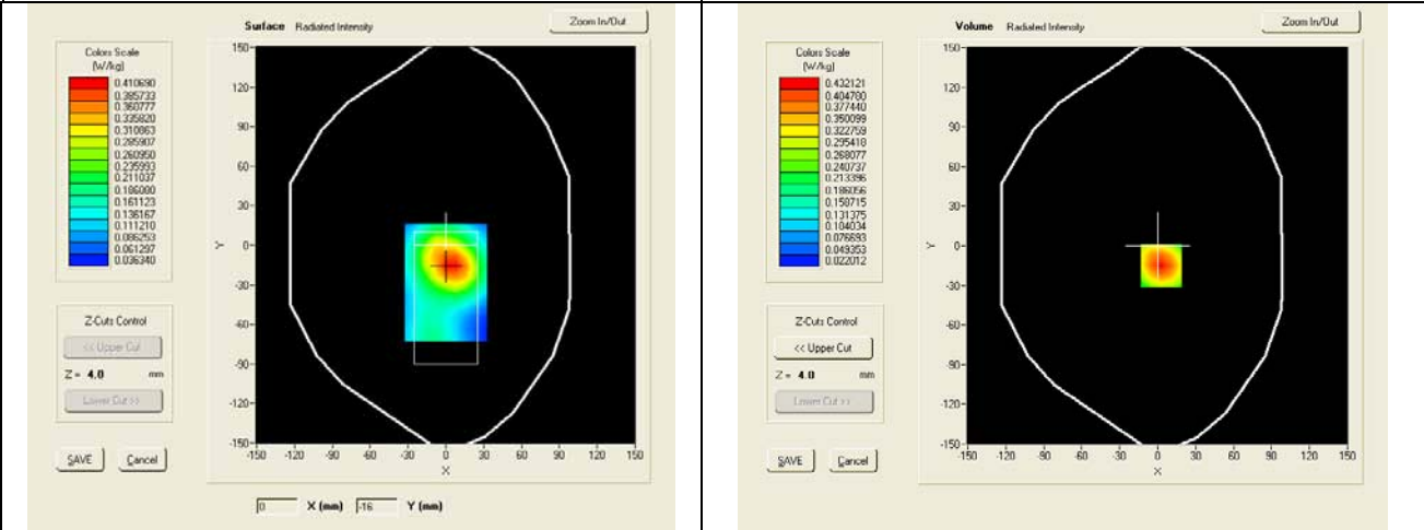
SAR, Z Axis Scan (X = 3, Y = -15)
