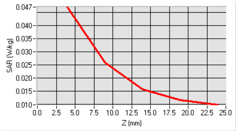
SAR, Z Axis Scan (X = -59, Y = -22)
