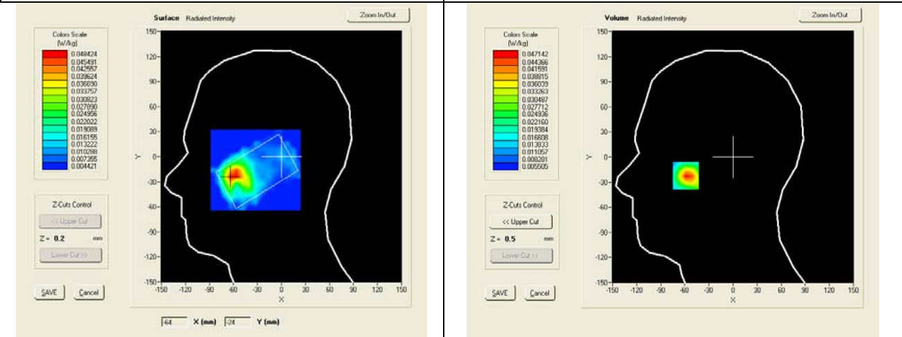
SAR, Z Axis Scan (X = -59, Y = -22)
