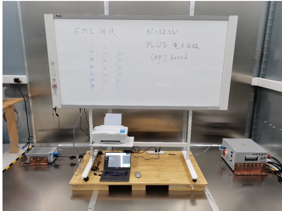
Photograph 4: Set-up for Radiated Emissions
