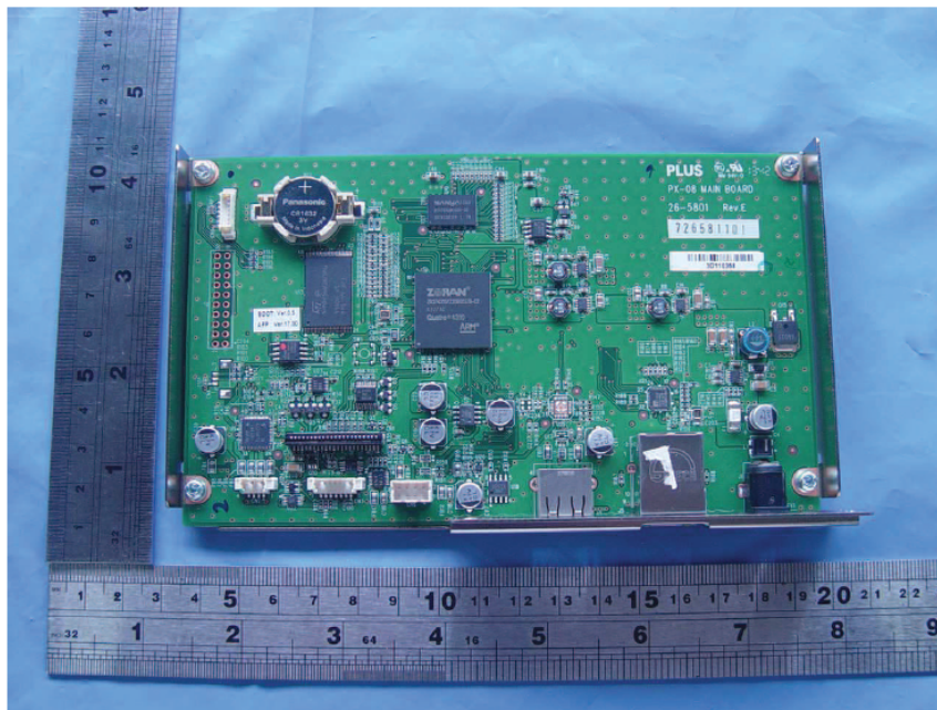
Figure 4: Main board top view
