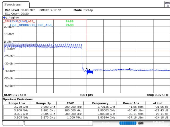
n78(3700-3800) SCS=30kHz DFT_BPSK BW=70MHz HighChannel=651000 RB=180@0
