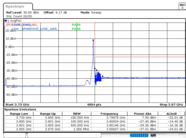
n78(3700-3800) SCS=30kHz DFT_16QAM BW=70MHz HighChannel=651000 RB=1@188
