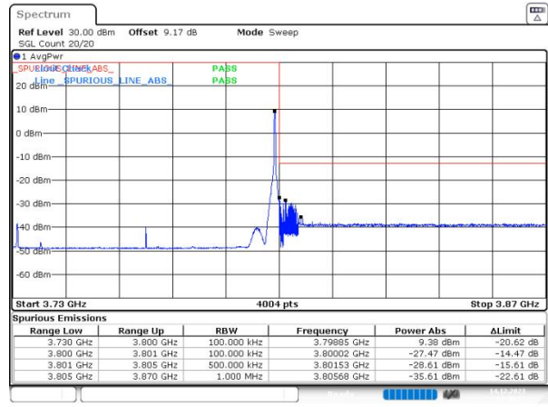
n78(3700-3800) SCS=30kHz DFT_QPSK BW=70MHz HighChannel=651000 RB=1@188
