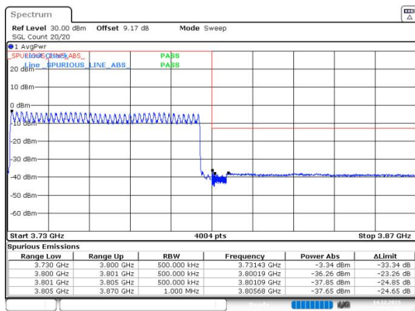
n78(3700-3800) SCS=30kHz DFT_QPSK BW=70MHz HighChannel=651000 RB=180@0
