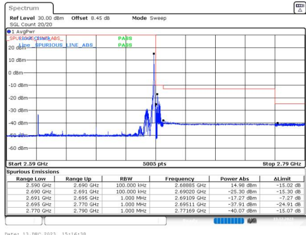
n41 SCS=30kHz DFT_BPSK BW=80MHz HighChannel=529998 RB=1@216
