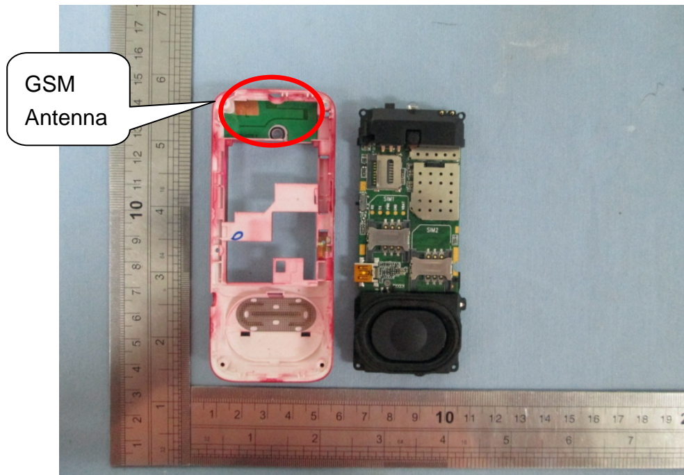
OPEN VIEW OF EUT-3
