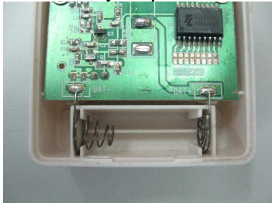
Battery Compartment
