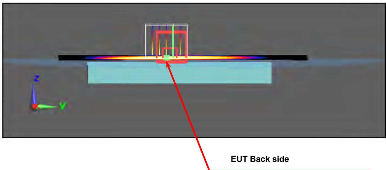
Figure 6. Body SAR Test Setup (Flat Section)
