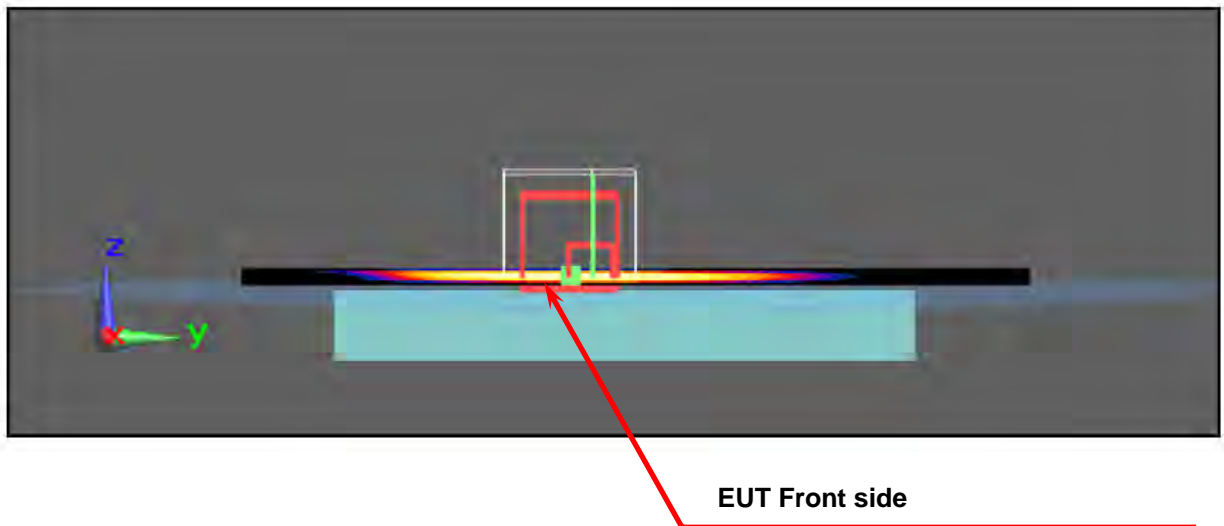
Figure 5. Body SAR Test Setup (Flat Section)
