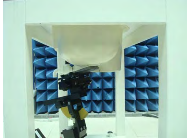
Figure 4. Left Head SAR Test Setup (Tilted)
