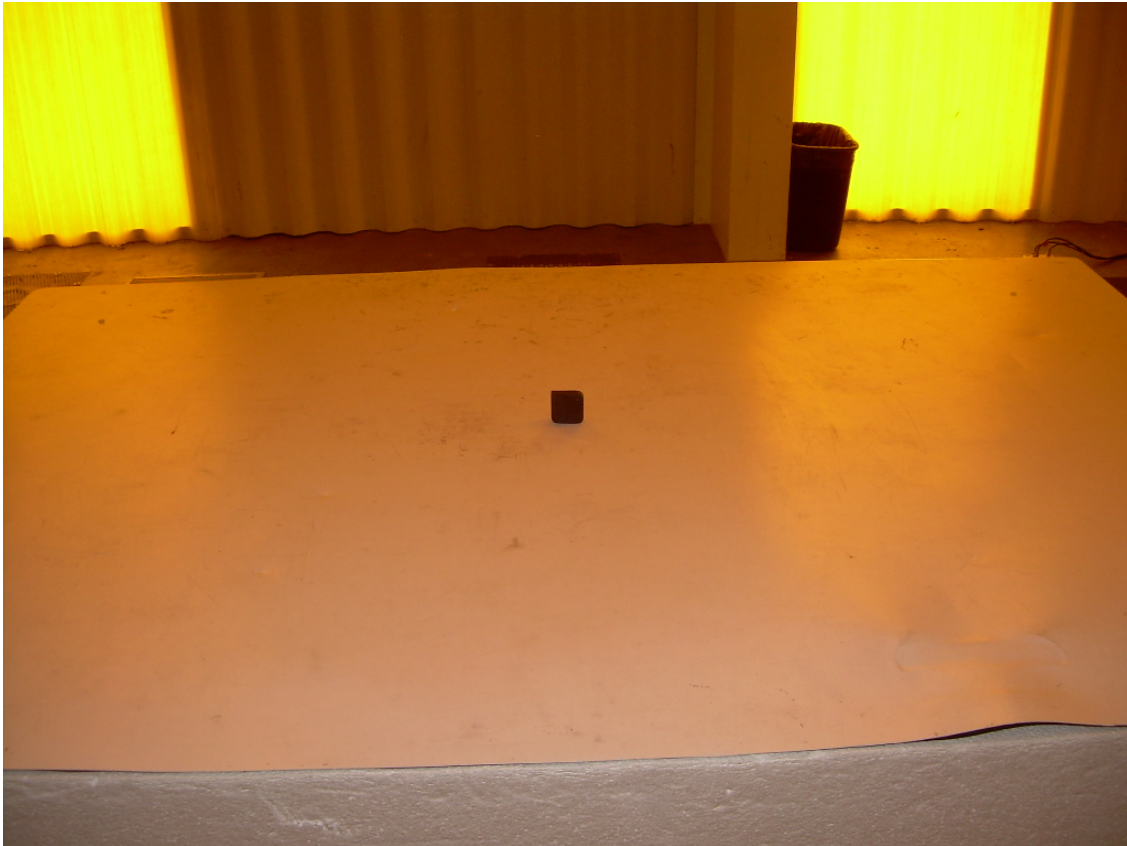
Photograph 2 – Radiated Disturbance Configuration – Vertical
