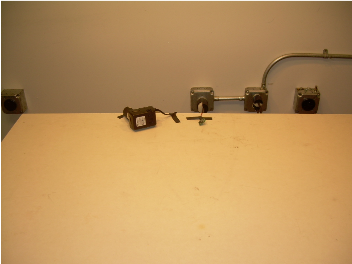
Photograph 5 – Front View Conducted Emission Configuration
