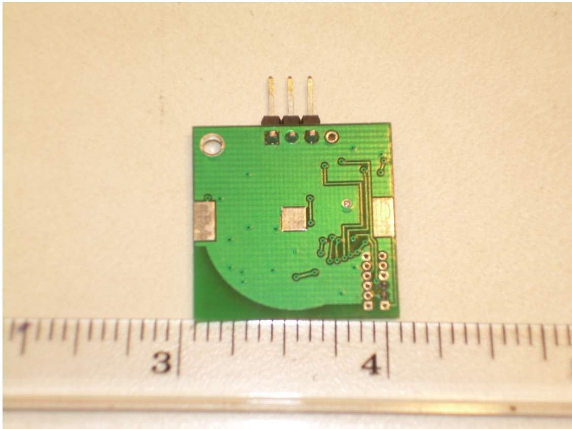
Photograph 8 – View of the Trace Side of the PCB – External Power Unit
