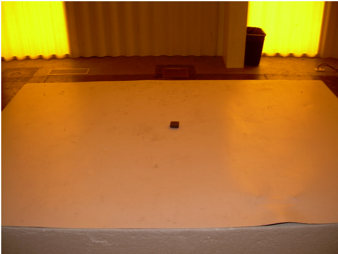
Photograph 1 – Radiated Disturbance Worst-Case Test Configuration - Horizontal
