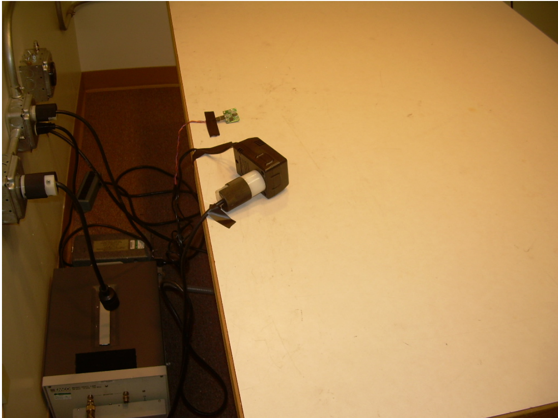
Photograph 6 – Back View Conducted Emission Configuration
