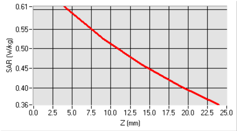
SAR, Z Axis Scan (X = -17, Y = -3)
