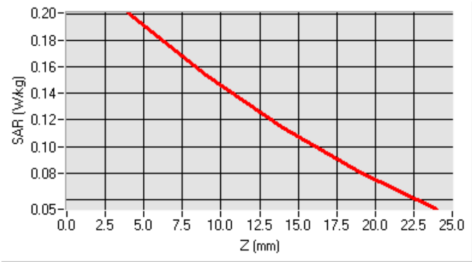
SAR, Z Axis Scan (X = 8, Y = -32)
