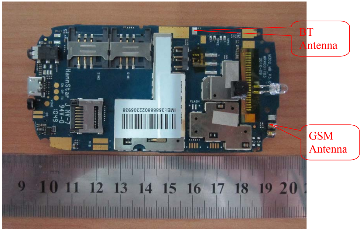
PCB Board view
