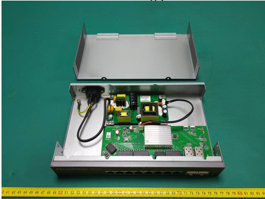
GOS Power Supply
