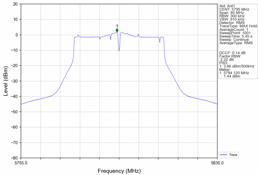
02.11ac(VHT40)_HCH_5795MHz_Ant1_NTNV
