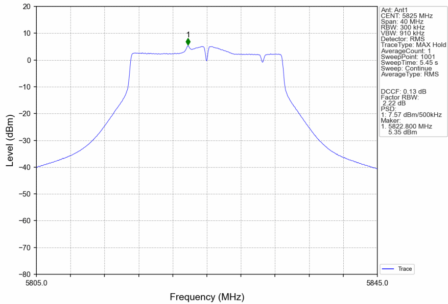
802.11ac(VHT20)_HCH_5825MHz_MIMO_NTNV
