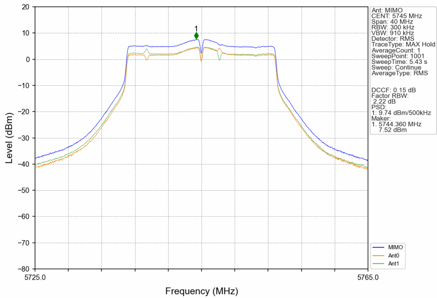
802.11ac(VHT20)_LCH_5745MHz_MIMO_NTNV
