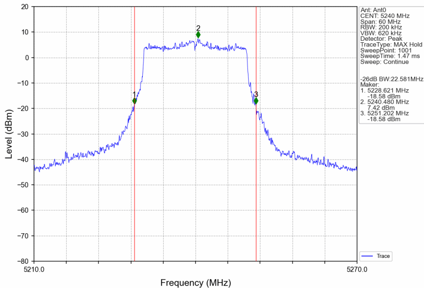
802.11ax(HEW20)_HCH_5240MHz_SU_ / _Ant0_NTNV
