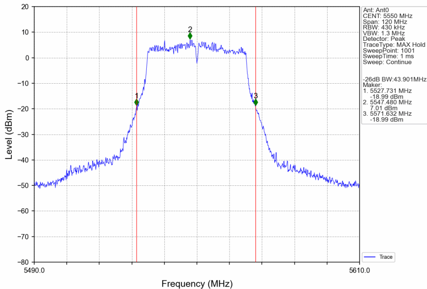
802.11ac(VHT40)_MCH_5550MHz_Ant0_NTNV
