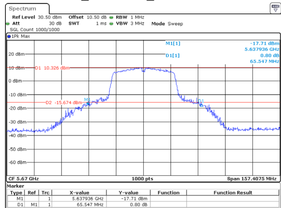
802.11ac40_5670MHz_Chain 0 65.547MHz
