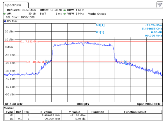
802.11ac80_5530MHz_Chain 2 99.099MHz
