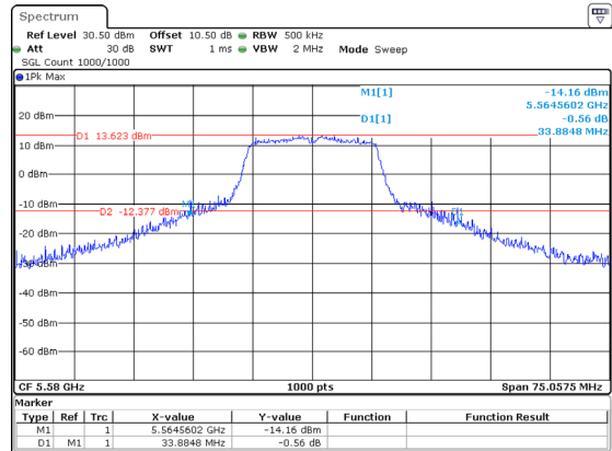
802.11a_5580MHz_Chain 2 33.885MHz
