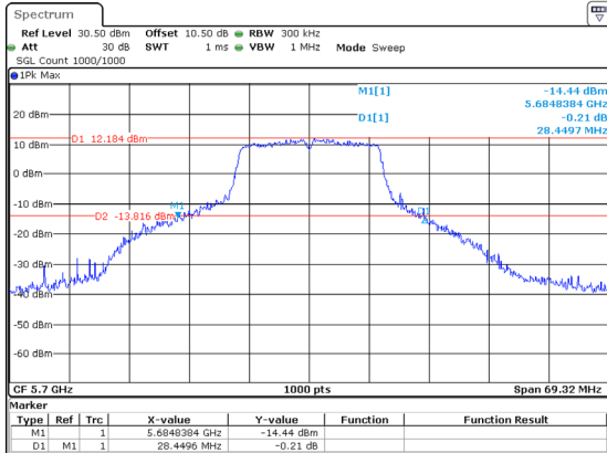
802.11a_5700MHz_Chain 1 28.450MHz
