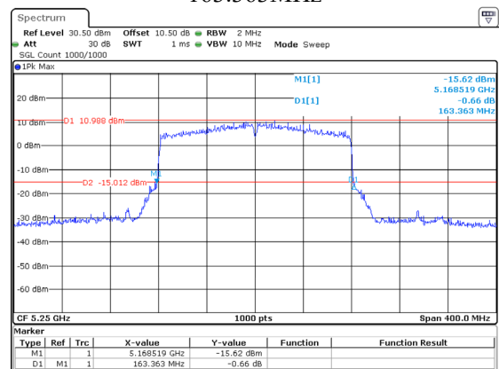
802.11ax160_5250MHz_RU_Full_Chain 0 163.363MHz
