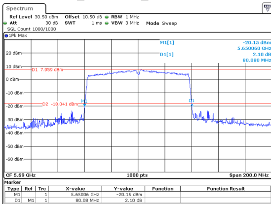
802.11ac80_5690MHz_Chain 1 80.080MHz
