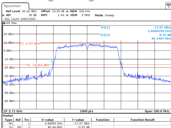
802.11ac40_5710MHz_Chain 1 40.440MHz
