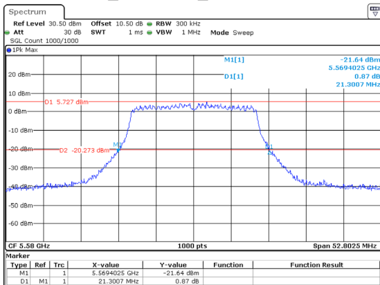
802.11ac20_5580MHz_Chain 1 21.301MHz
