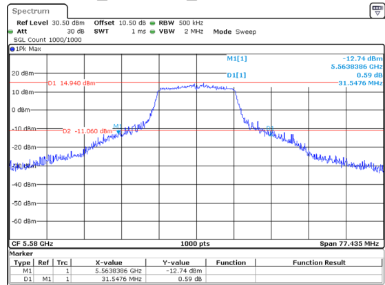
802.11a_5580MHz_Chain 0 31.548MHz
