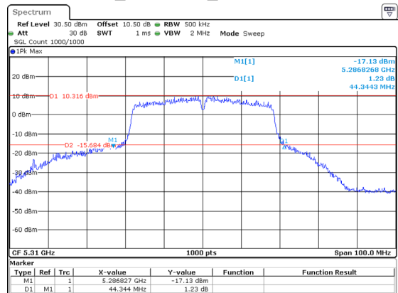
802.11ac40_5310MHz_Chain 1 44.344MHz
