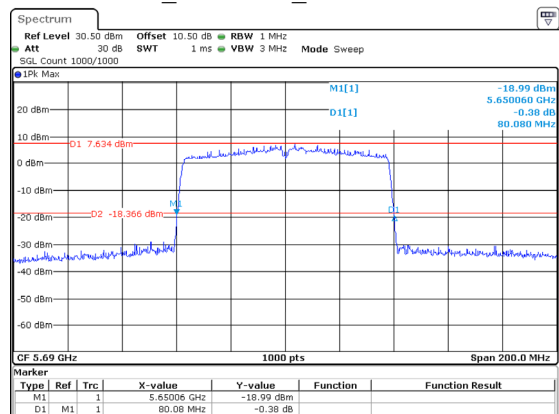
802.11ac80_5690MHz_Chain 2 80.080MHz
