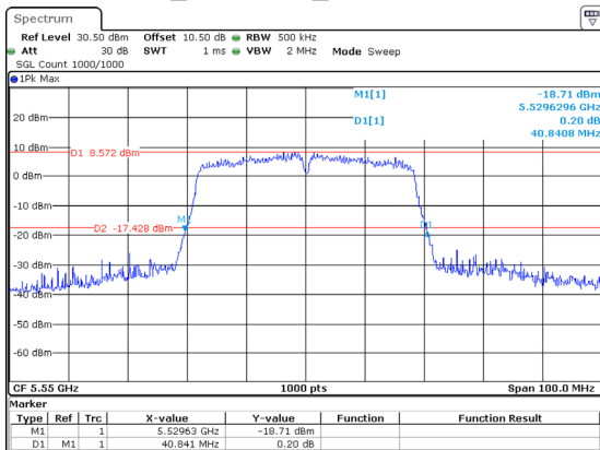
802.11ac40_5550MHz_Chain 1 40.841MHz
