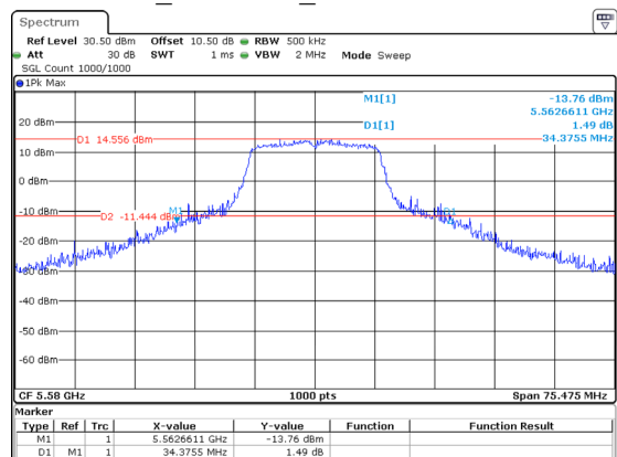
802.11a_5580MHz_Chain 1 34.376MHz
