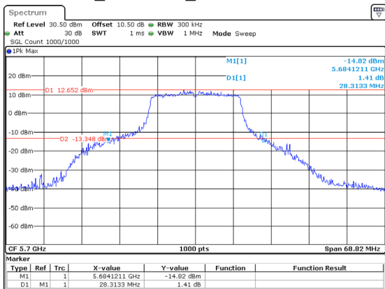
802.11a_5700MHz_Chain 0 28.313MHz
