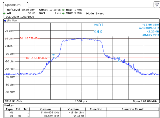
802.11ac40_5510MHz_Chain 0 58.669MHz
