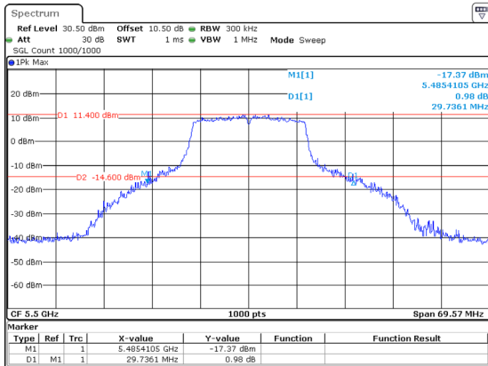
802.11a_5500MHz_Chain 2 29.736MHz
