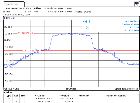
802.11ac40_5670MHz_Chain 1 62.876MHz
