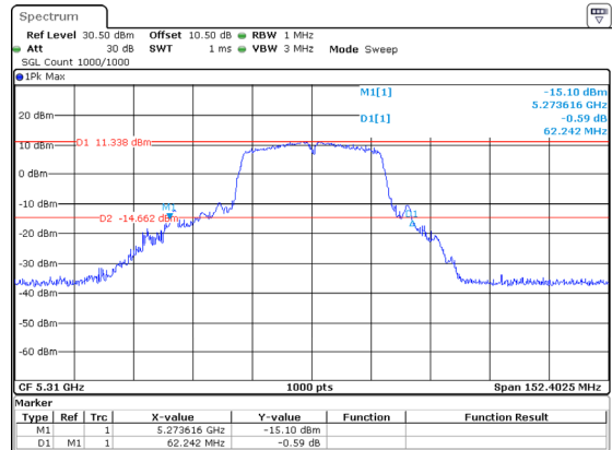
802.11ac40_5310MHz_Chain 0 62.242MHz
