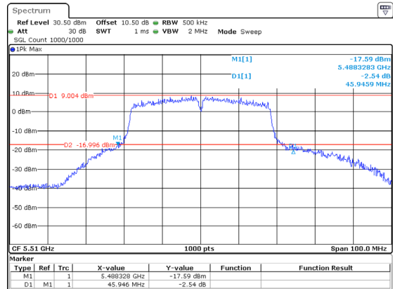
802.11ac40_5510MHz_Chain 1 45.946MHz
