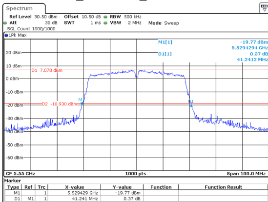
802.11ac40_5550MHz_Chain 0 41.241MHz
