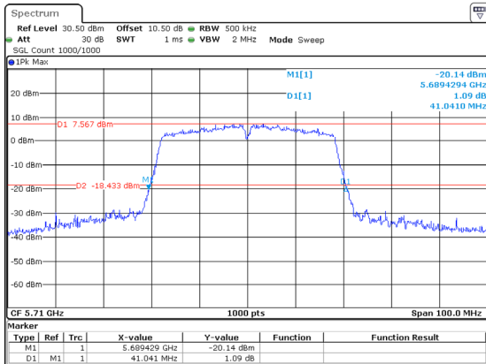
802.11ac40_5710MHz_Chain 0 41.041MHz
