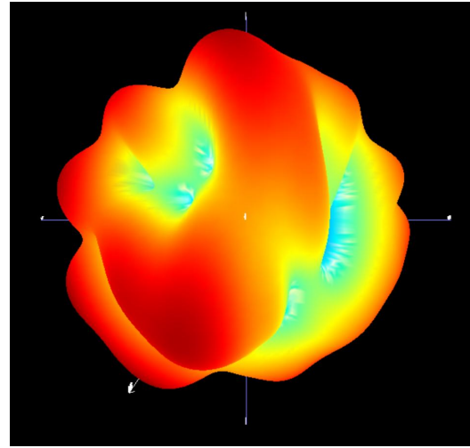
2.4G 3D
