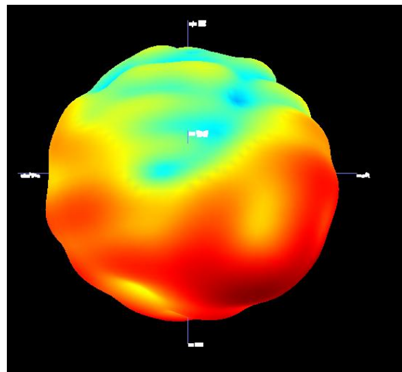
5G 3D
