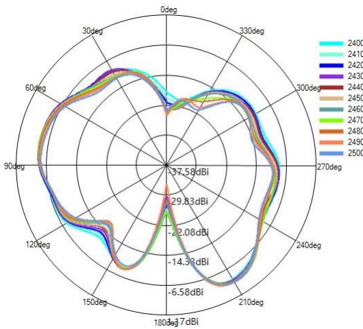
2.4G phi=90deg
