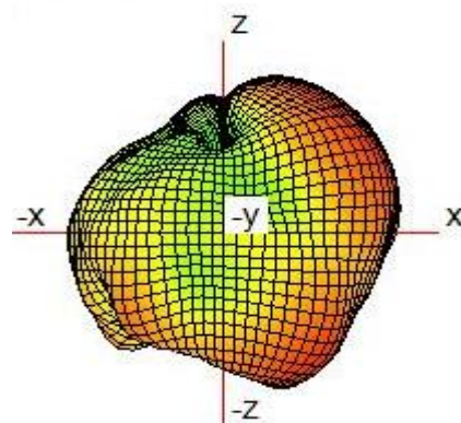
2.4G 3D
