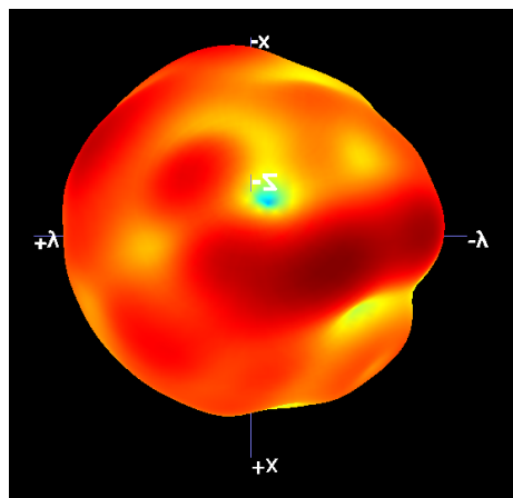
2.4G 3D
