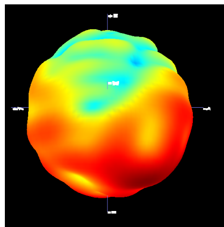
5G 3D
