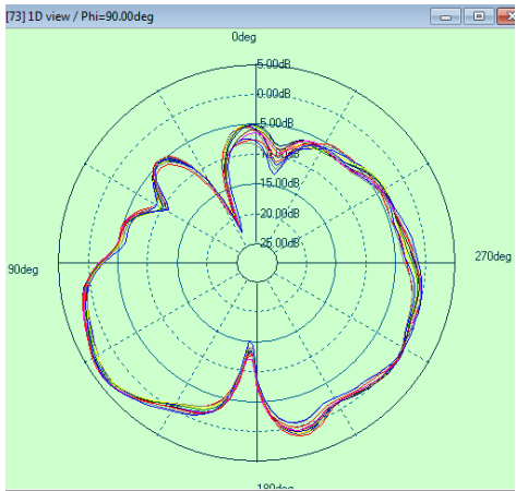
2.4G phi=90deg
