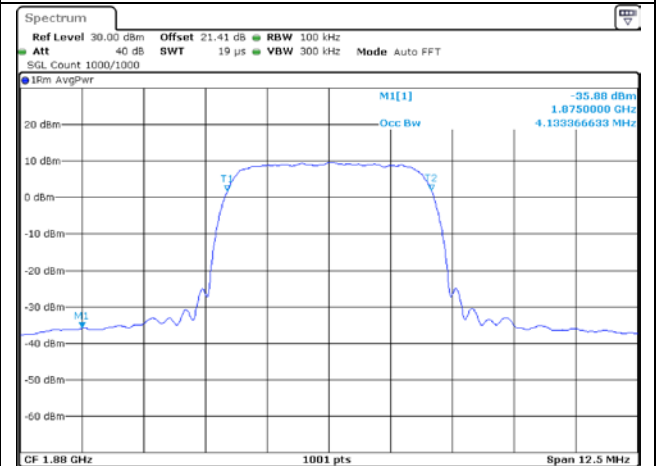
Low Channel (99 % Occupied Bandwidth)
