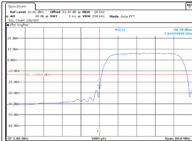
Low Channel (RMC)
