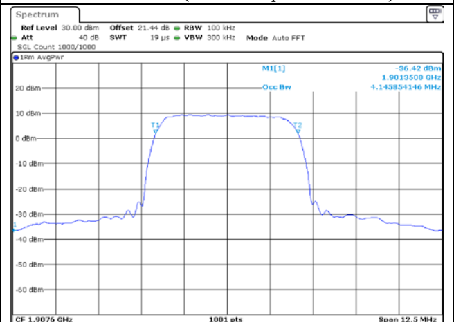
Middle Channel (99 % Occupied Bandwidth)
