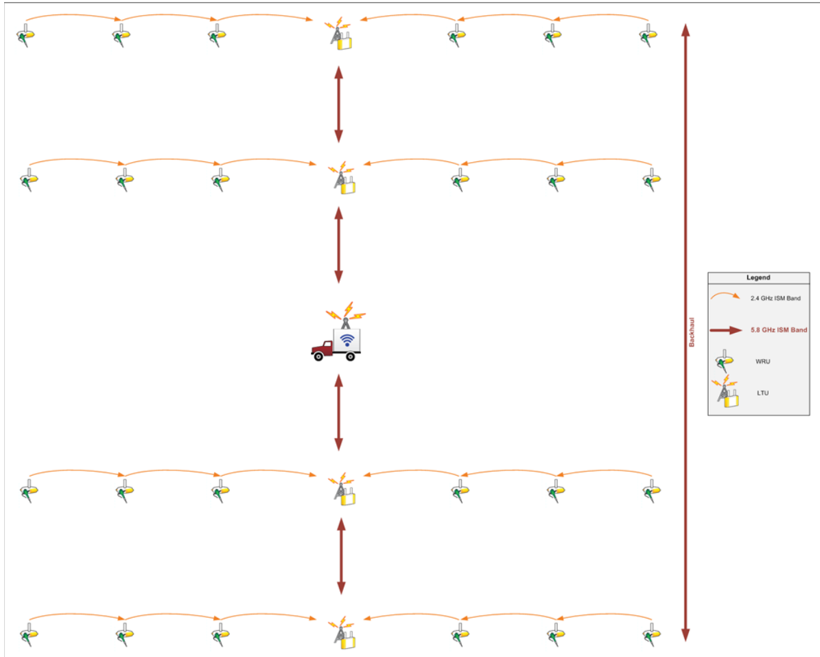
Figure 3–33 2D Single Backhaul
