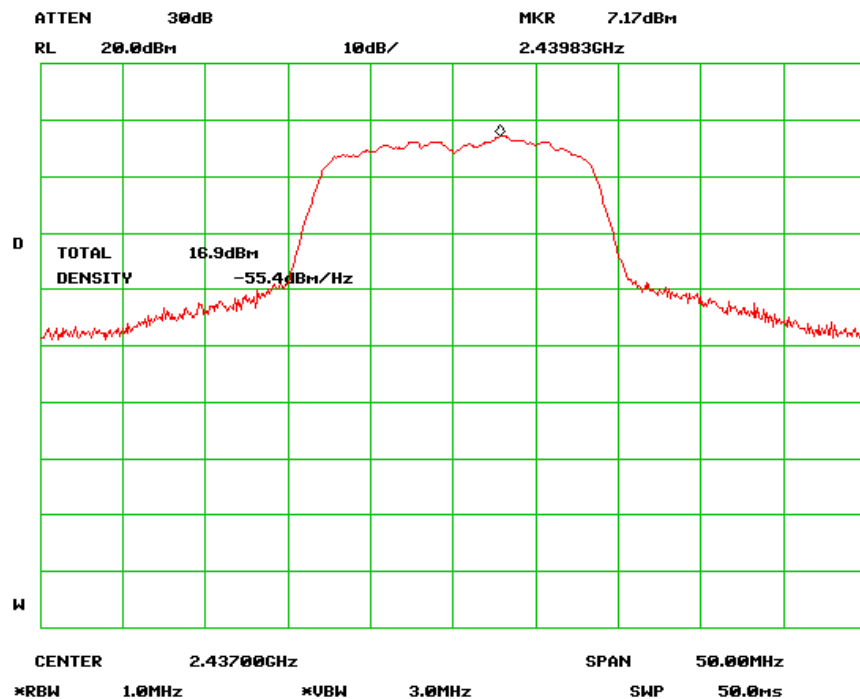
Peak Output Power - Mid Channel (802.11g)
