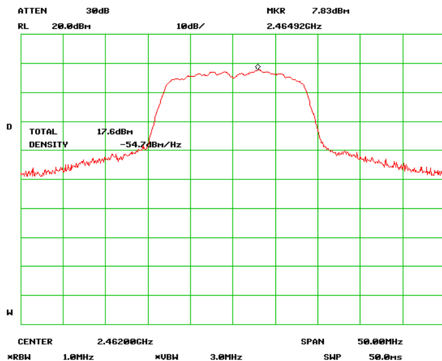
Peak Output Power - High Channel (802.11g)
