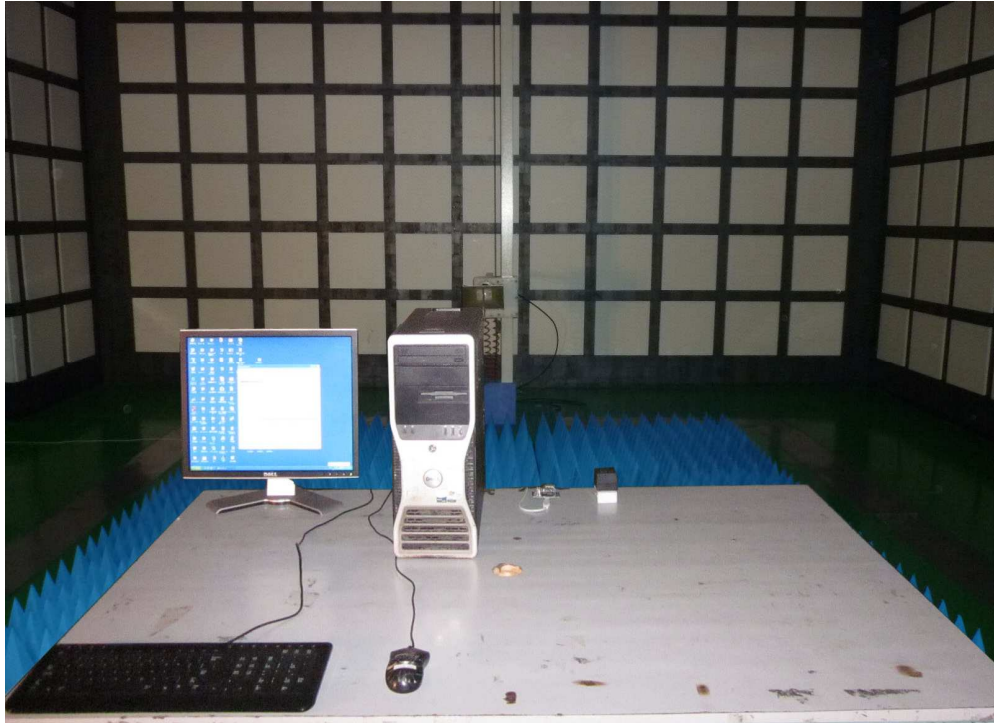
Photograph 3: Set-up for Spurious Emissions 1GHz – 26.5GHz
