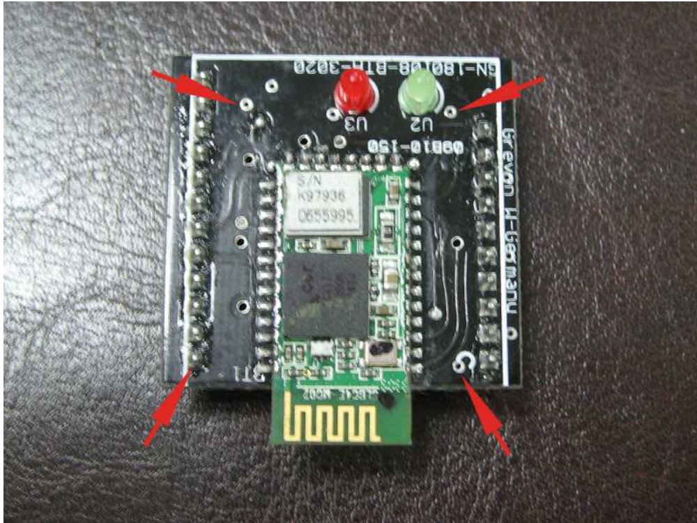
Top side-the solder points are marked with red array
