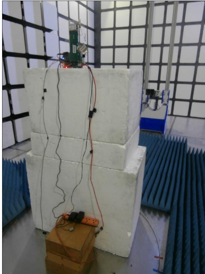
Figure 5 - Radiated Emissions - 1 GHz to 8 GHz - Y Orientation
