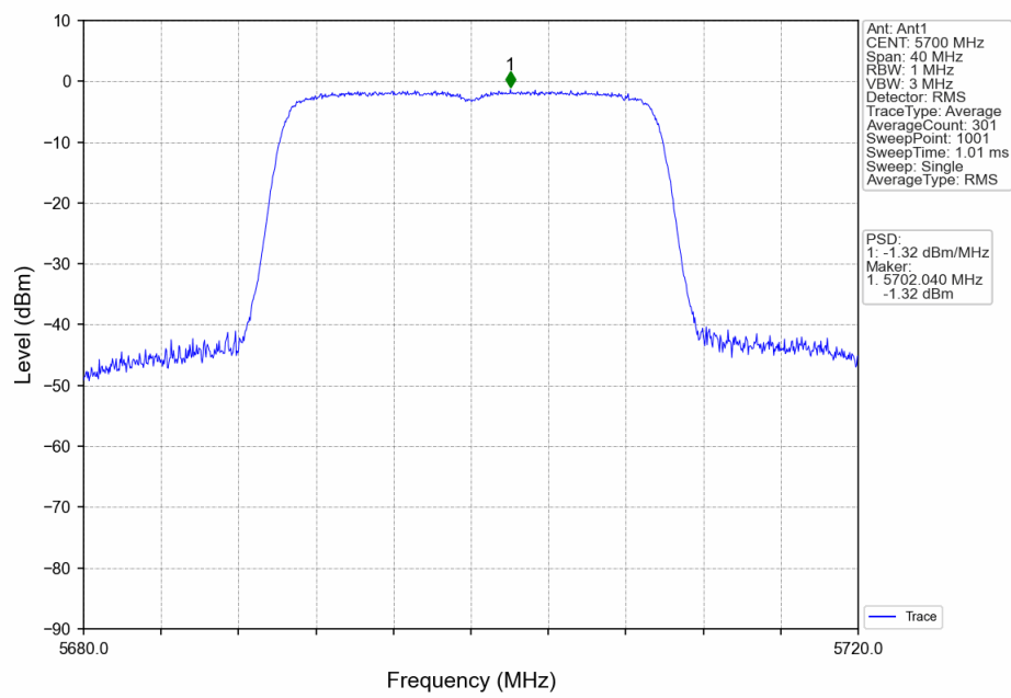
802.11ax(HEW20)_HCH_5700MHz_RU242_Left_Ant1_NTNV
