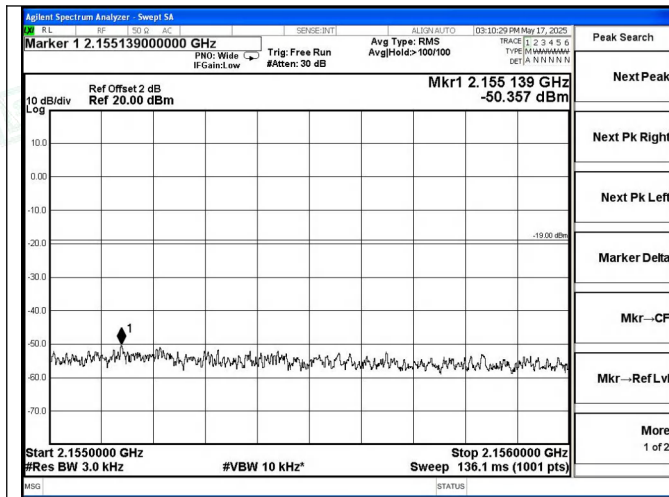
AWS Band DL-LTE Right Side Pre AGC
