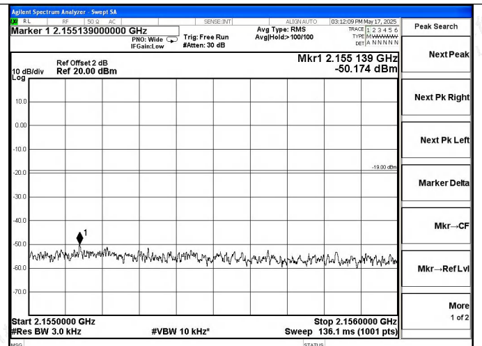
AWS Band DL-LTE Right Side AGC+5.5dB
