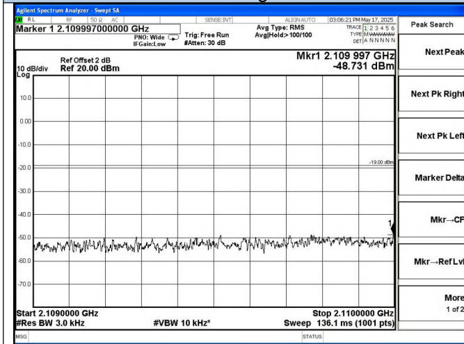
AWS Band DL-LTE Left Side Pre AGC
