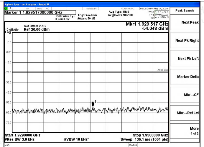
PCS Band DL-LTE Left Side AGC+5.5dB
