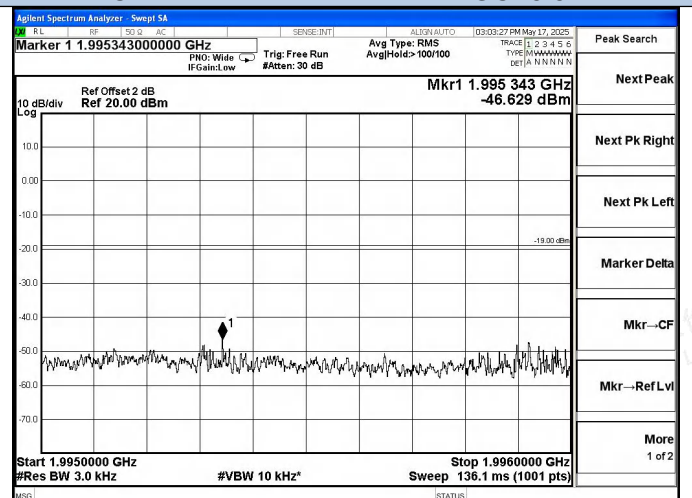
PCS Band DL-LTE Right Side AGC+5.5dB
