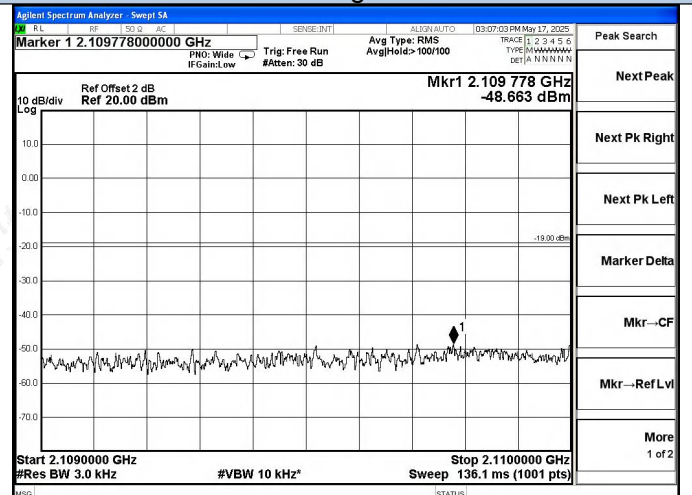
AWS Band DL-LTE Left Side AGC+5.5dB
