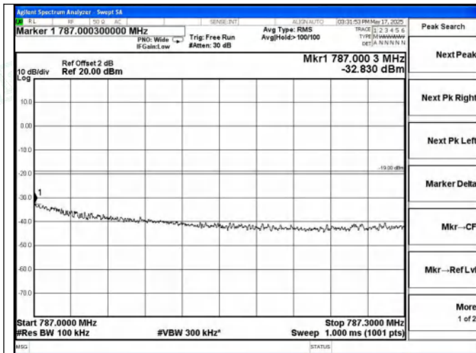
Upper 700 Band UL-LTE Right Side Pre AGC
