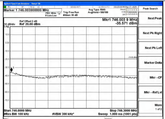
Lower 700 Band DL-LTE Right Side AGC+5.5dB
