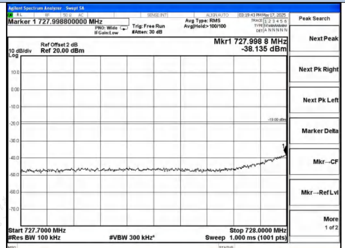
Lower 700 Band DL-LTE Left Side AGC+5.5dB
