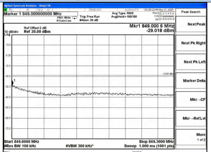
Cellular Band UL-LTE Right Side AGC+5.5dB
