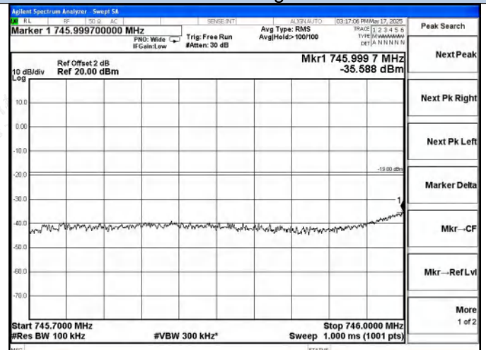
Upper 700 Band DL-LTE Left Side AGC+5.5dB
