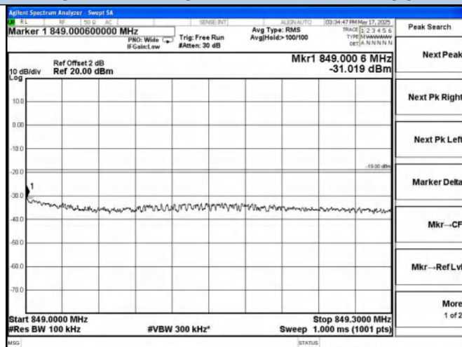
Cellular Band UL-LTE Right Side Pre AGC
