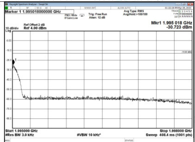
PCS Band GSM DL Right Side 10dB Above AGC
