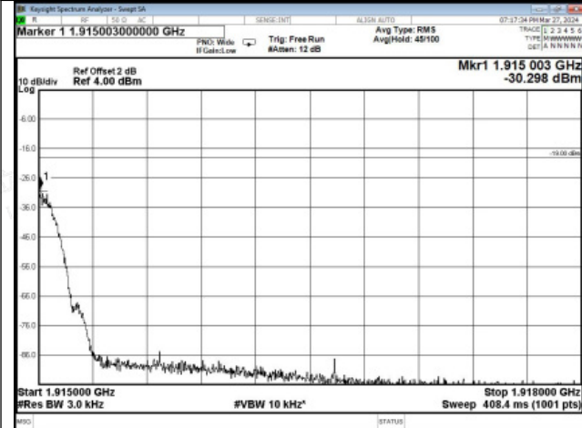
PCS Band GSM UL Right Side Pre AGC
