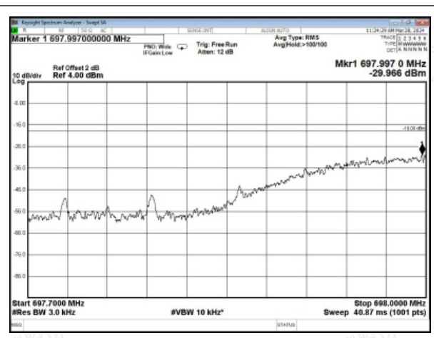
Lower 700MHz band GSM UL Left Side 10dB Above AGC
