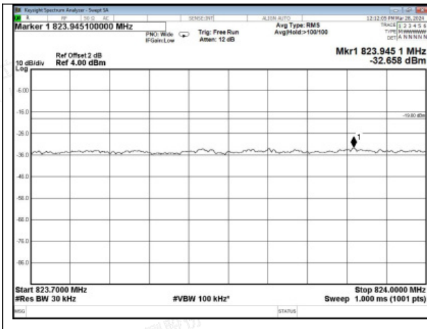
Cellular Band CDMA UL Left Side Pre AGC
