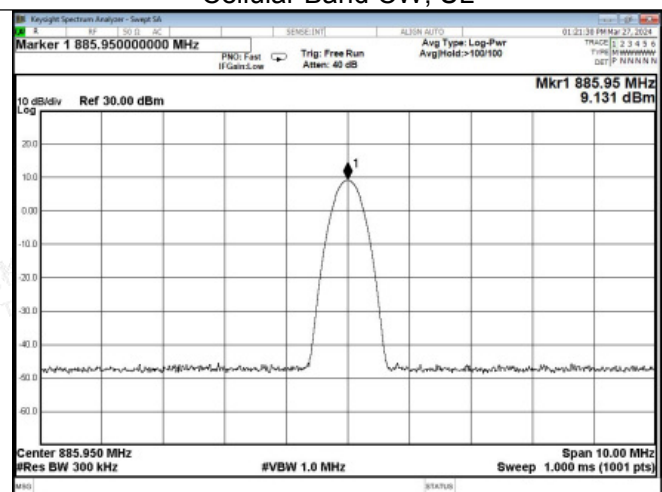
Cellular Band CW, DL
