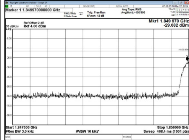
PCS Band GSM UL Left Side Pre AGC
