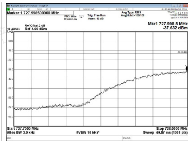
Lower 700MHz band GSM DL Left Side Pre AGC
