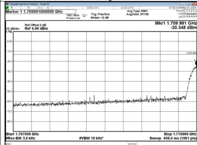
AWS Band GSM UL Left Side Pre AGC
