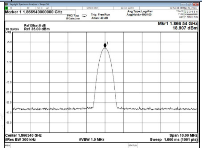
PCS Band CW, UL
