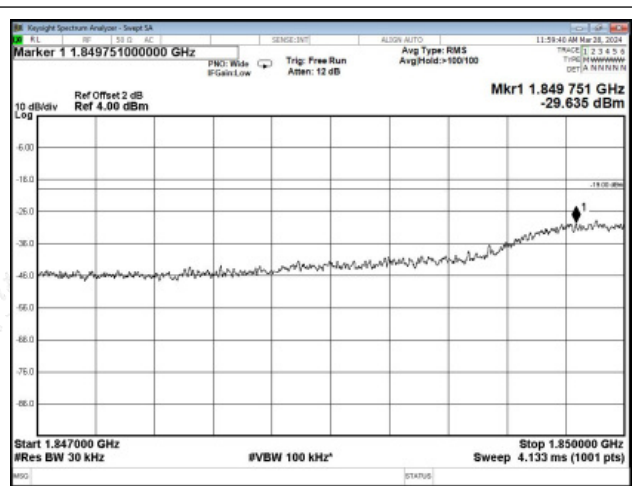
PCS Band CDMA UL Left Side 10dB Above AGC
