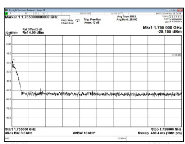
AWS Band GSM UL Right Side 10dB Above AGC
