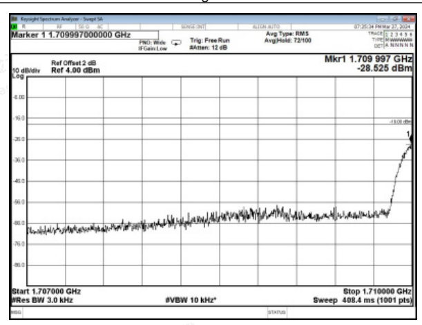
AWS Band GSM UL Left Side 10dB Above AGC
