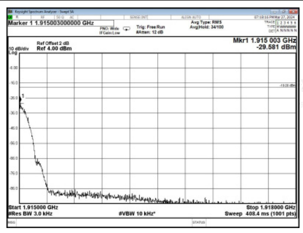
PCS Band GSM UL Right Side 10dB Above AGC
