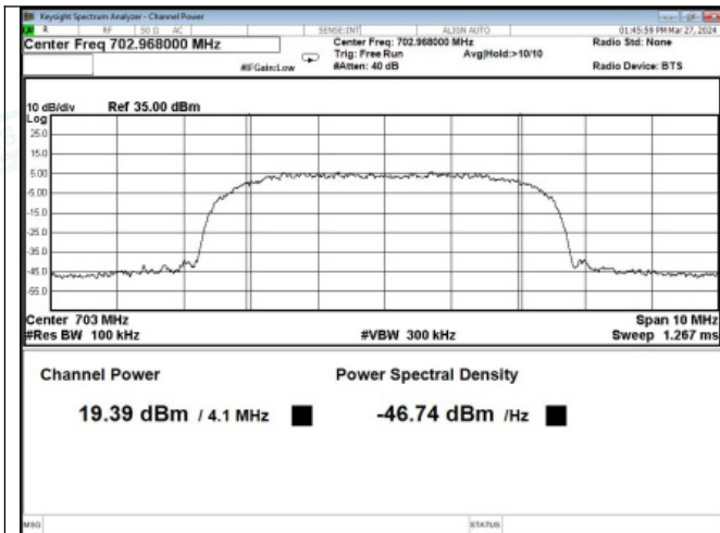
Lower 700MHz Band AWGN, UL
