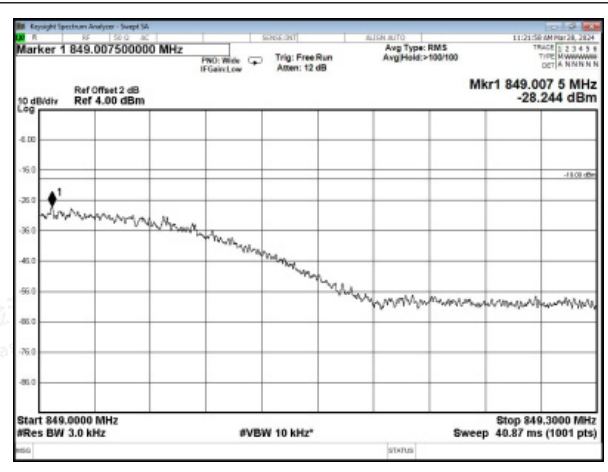
Cellular Band GSM UL Right Side 10dB Above AGC
