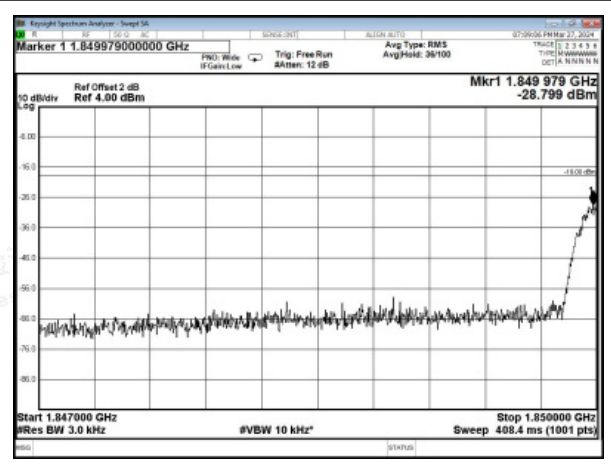
PCS Band GSM UL Left Side 10dB Above AGC
