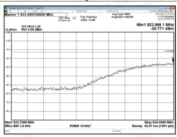
Cellular Band GSM UL Left Side 10dB Above AGC
