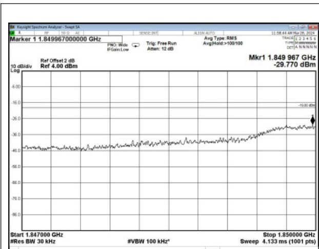
PCS Band CDMA UL Left Side Pre AGC
