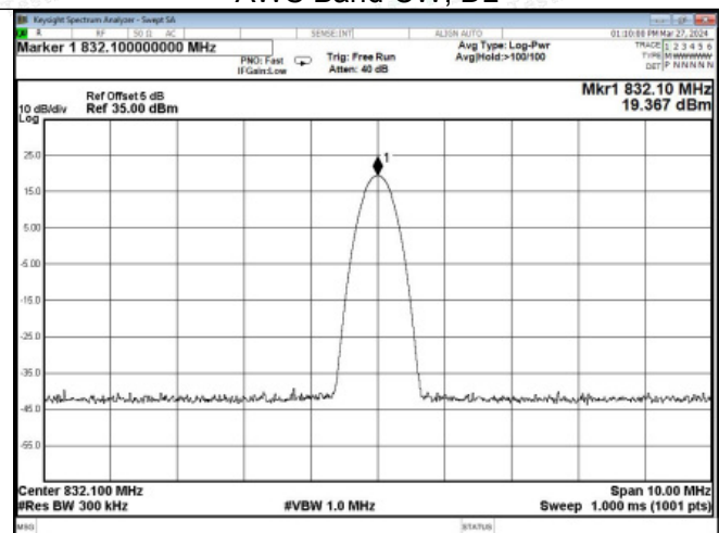
Cellular Band CW, UL
