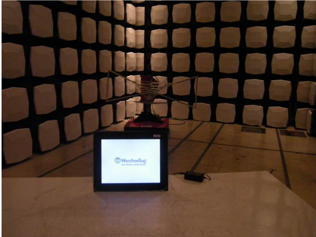
Radiated Measurement(15')
