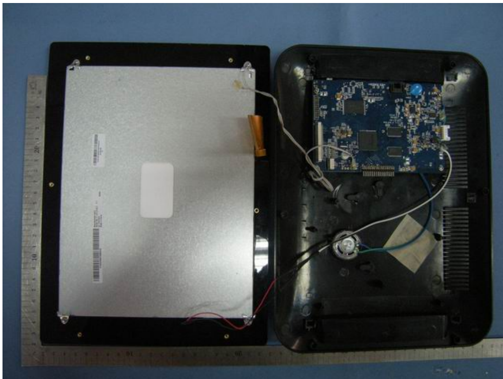
Internal photos of SCD10-1210S (10.4")
