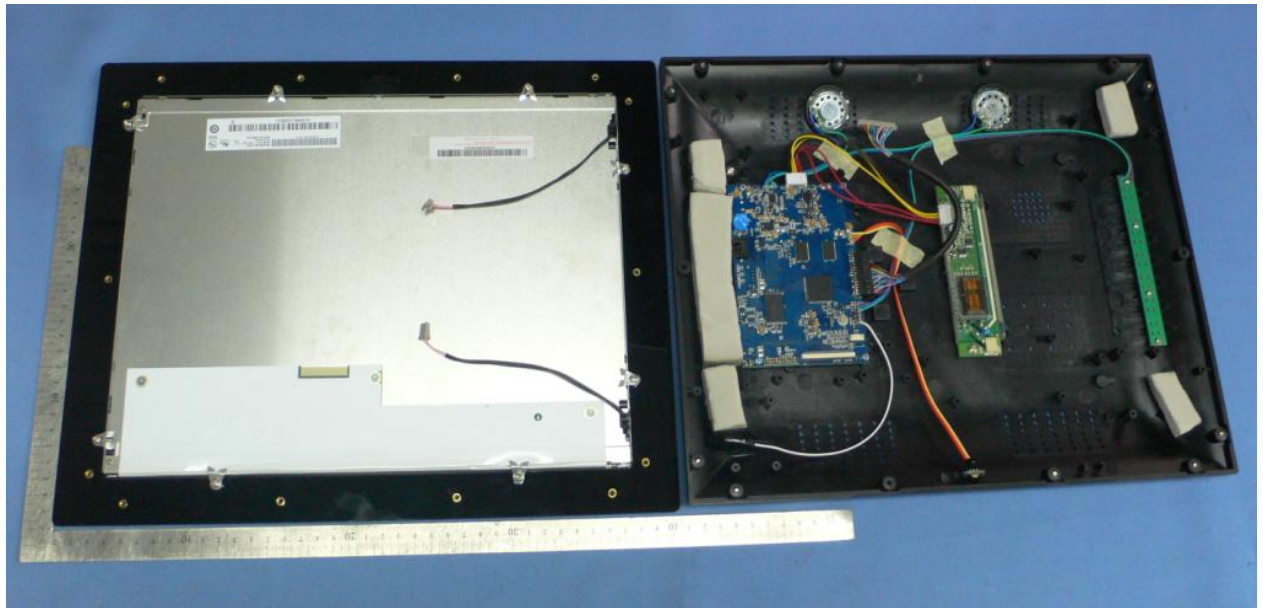
Internal photos of SCD15-1210S (15")
