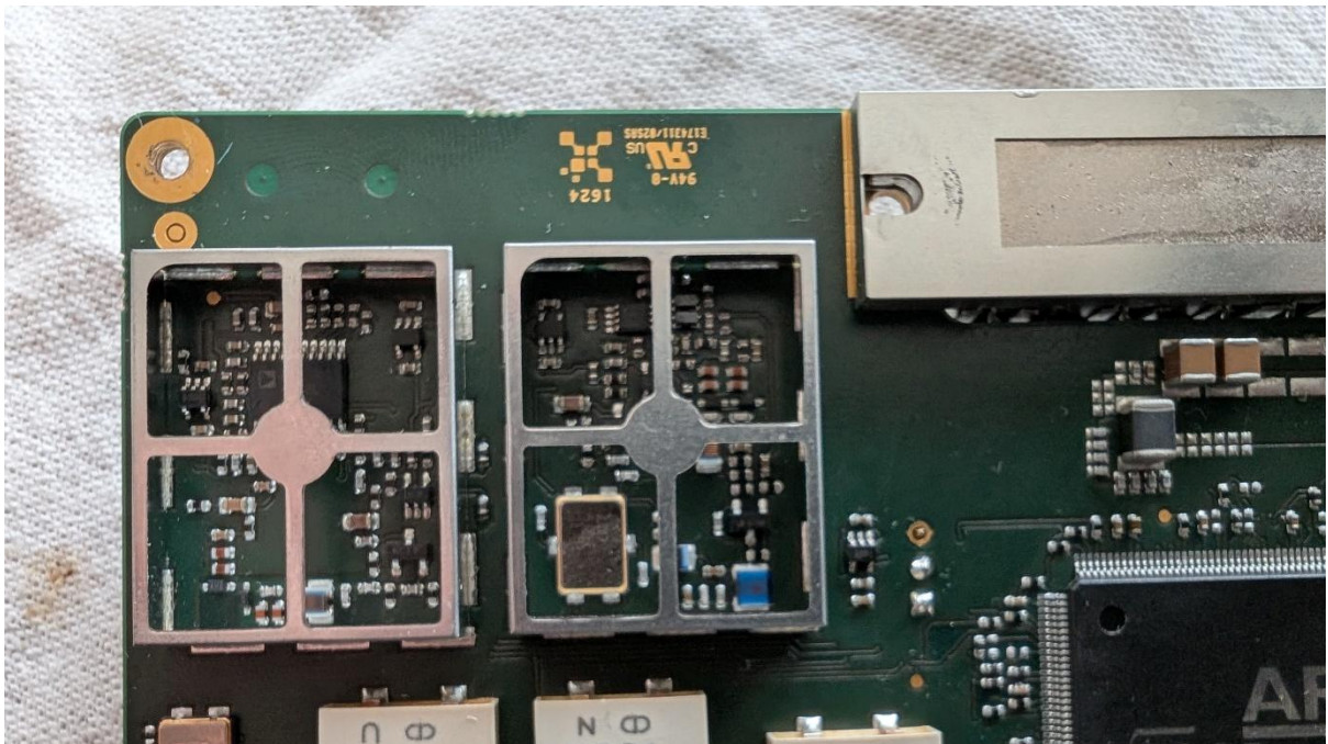
Main PCA bottom can close up
