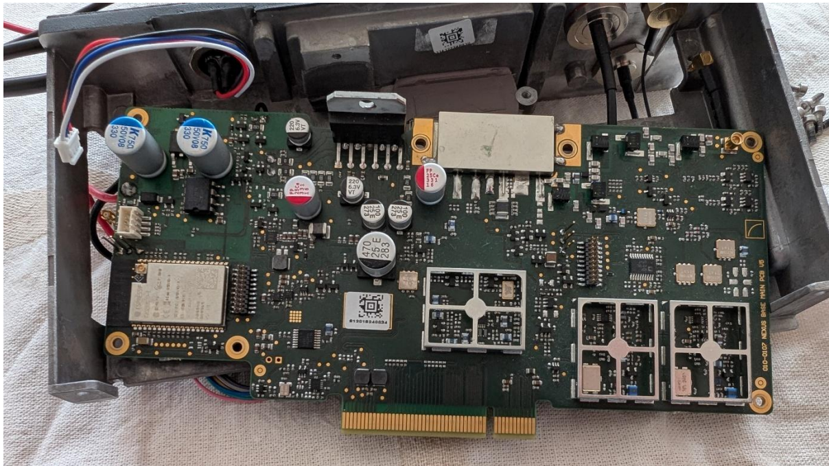
Main PCA without cans
