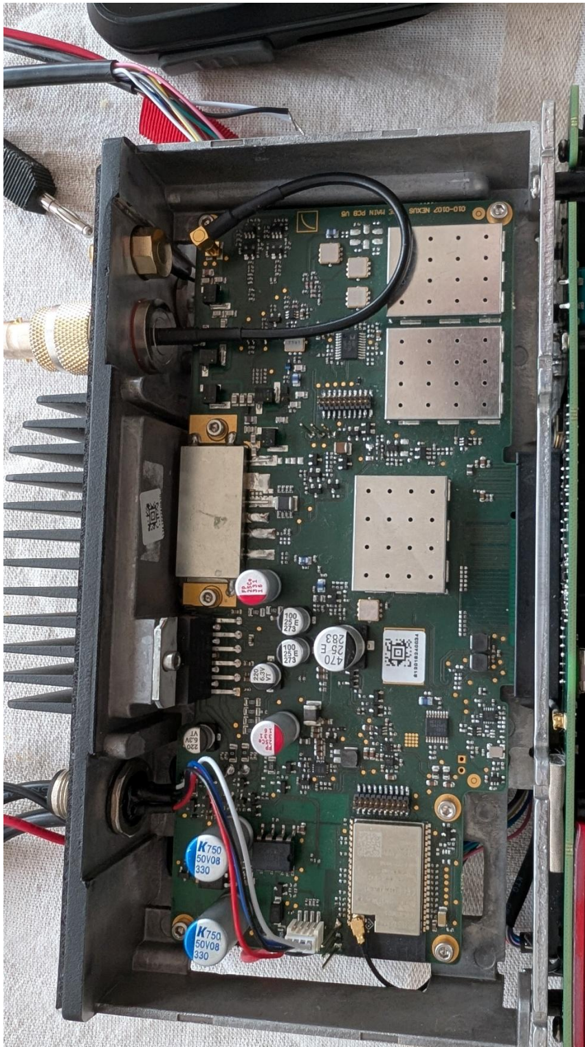
Main Chassis and HMI chassis fitted
