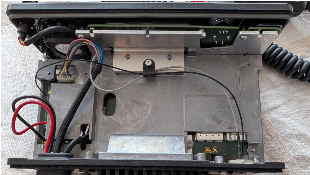
Main chassis and HMI chassis bottom
