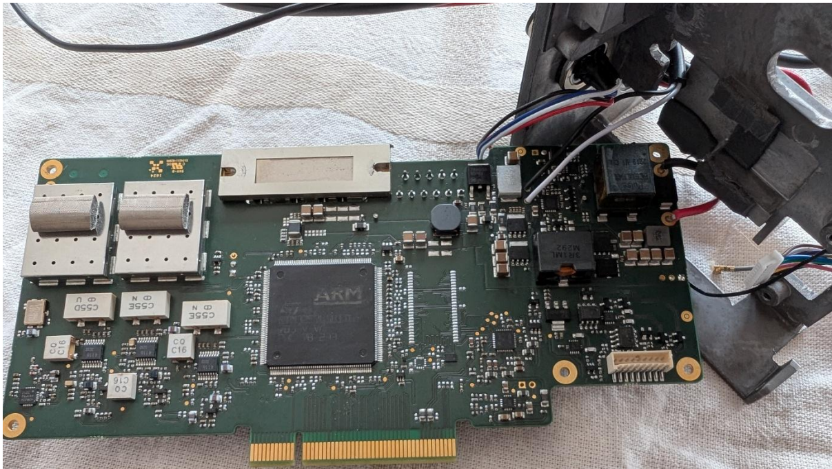
Main PCA bottom with cans
