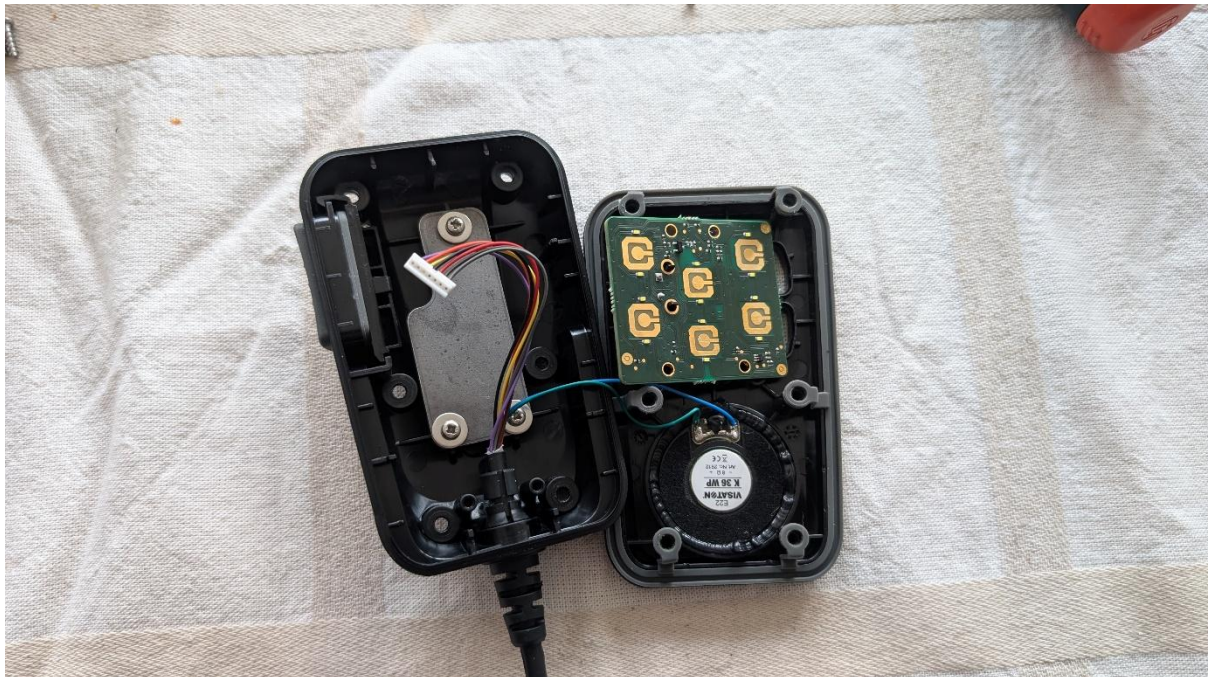
X100 fist mic PCA front
