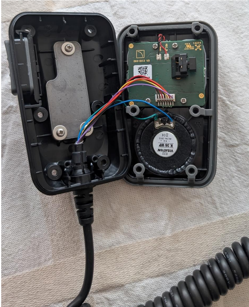
X100 fist mic PCA rear
