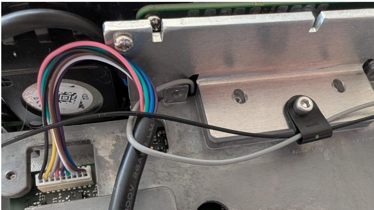
Main chassis and HMI chassis bottom GNSS cable location
