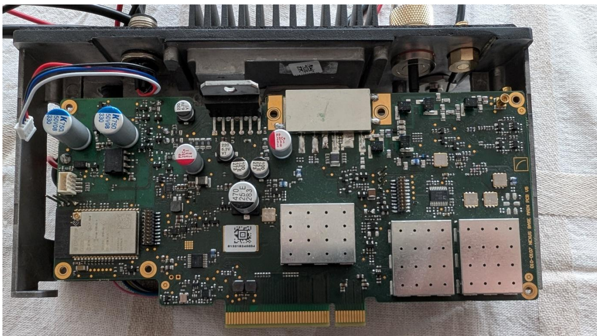
Main PCA top with cans
