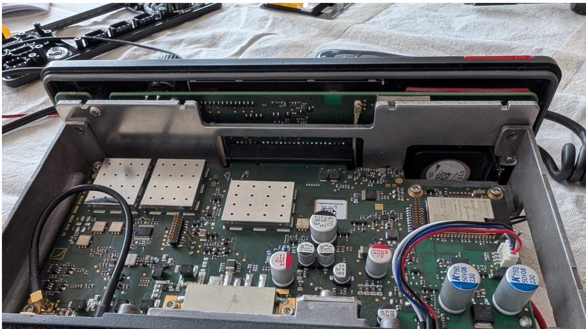
Main chassis and HMI chassis alt angle for cable view
