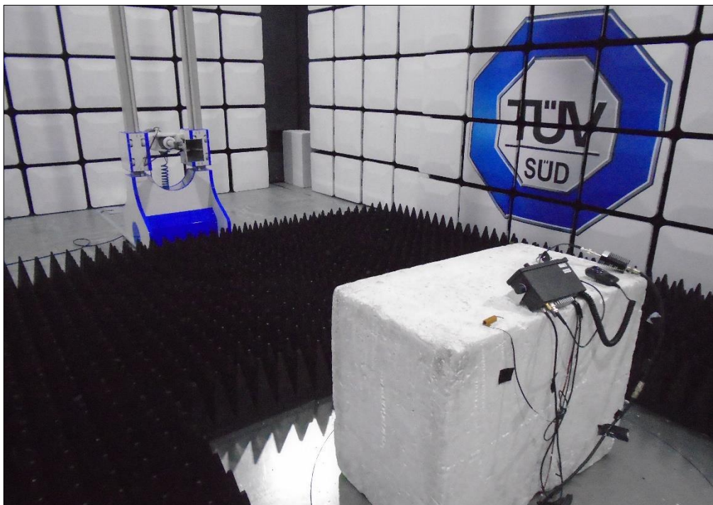
Figure 2 – Radiated Emissions - 1 MHz to 12 GHz
