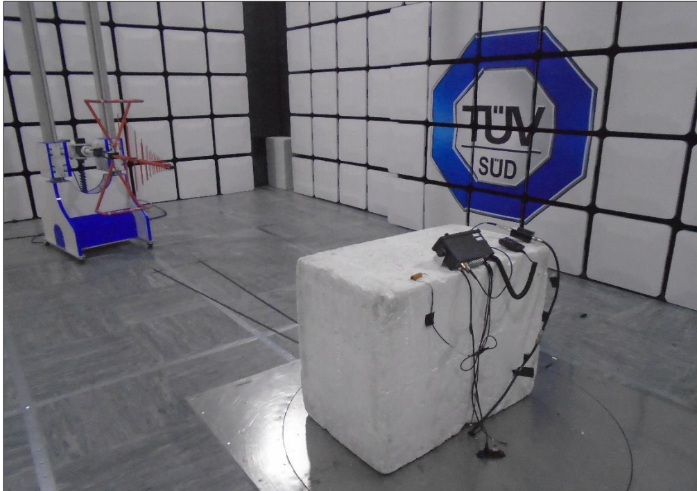
Figure 1 – Radiated Emissions - 30 MHz to 1 GHz
