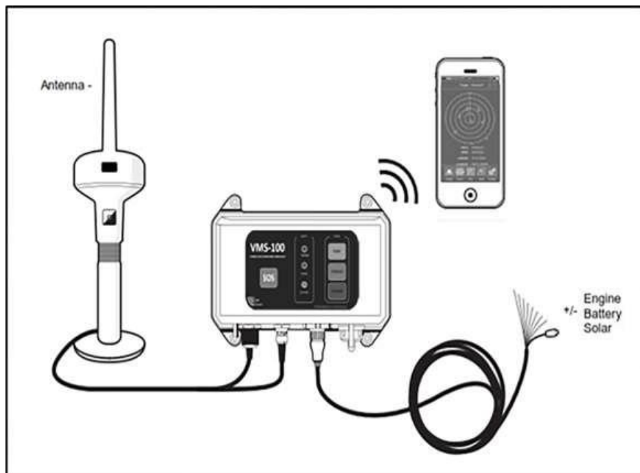
Figure 1 – VMS-100 System
