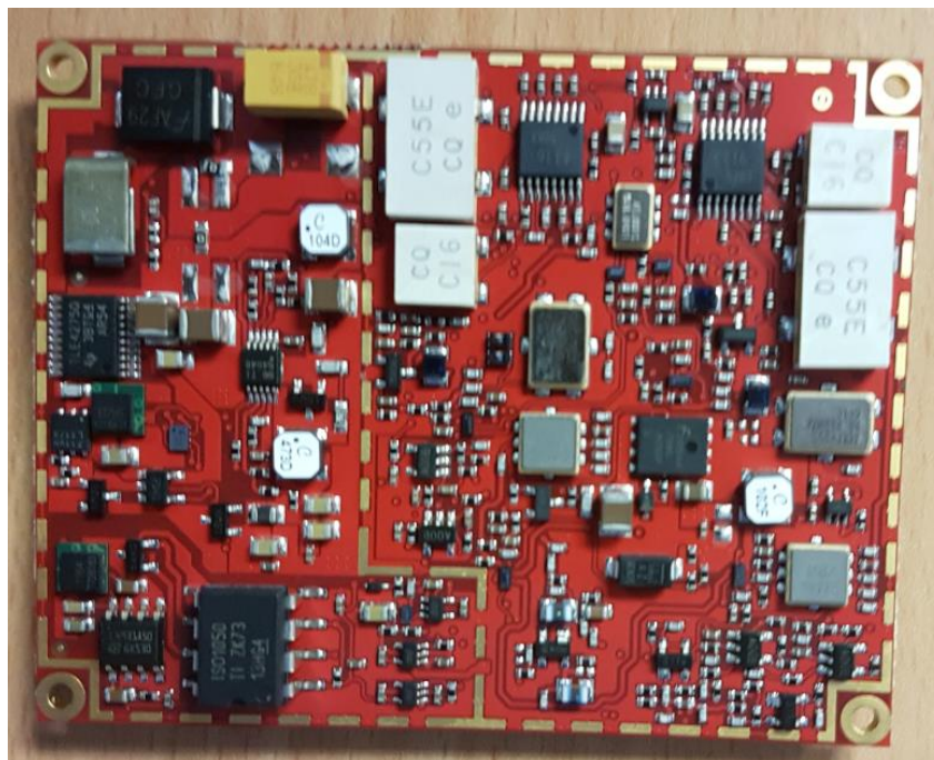
2. PCB Bottom
