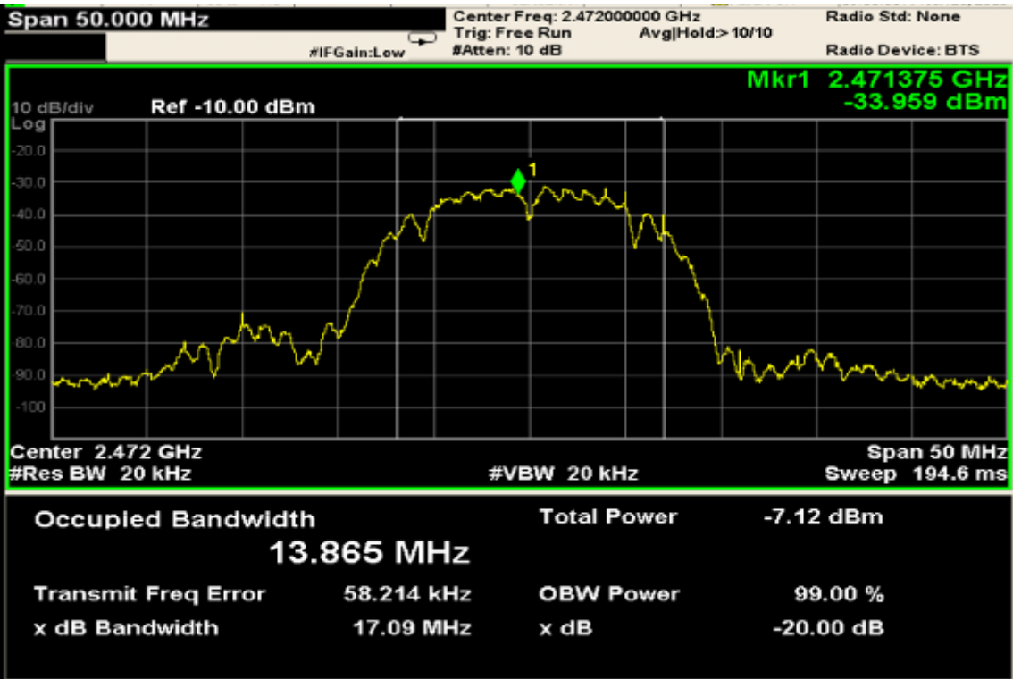
802.11b channel 13
