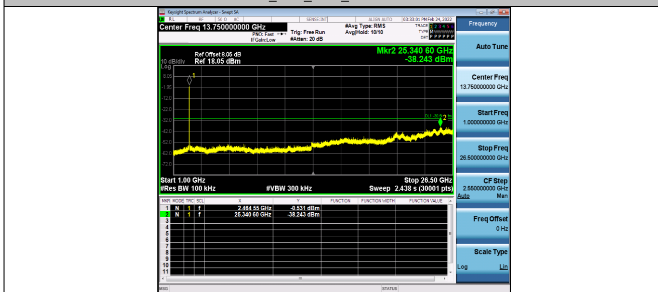
11N20SISO_Ant1_2412_0-Reference
