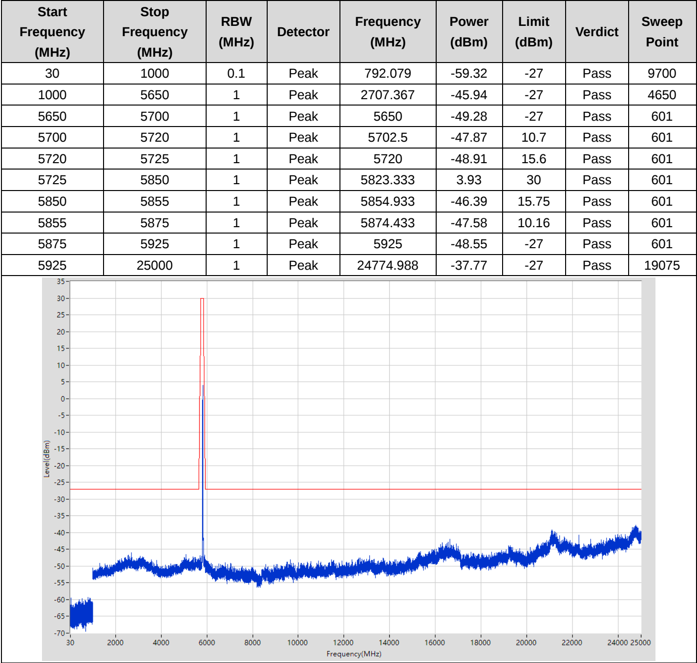
Figure 101: The Plots of conducted spurious emission, 802.11a20, 5825MHz, at Chain 1
