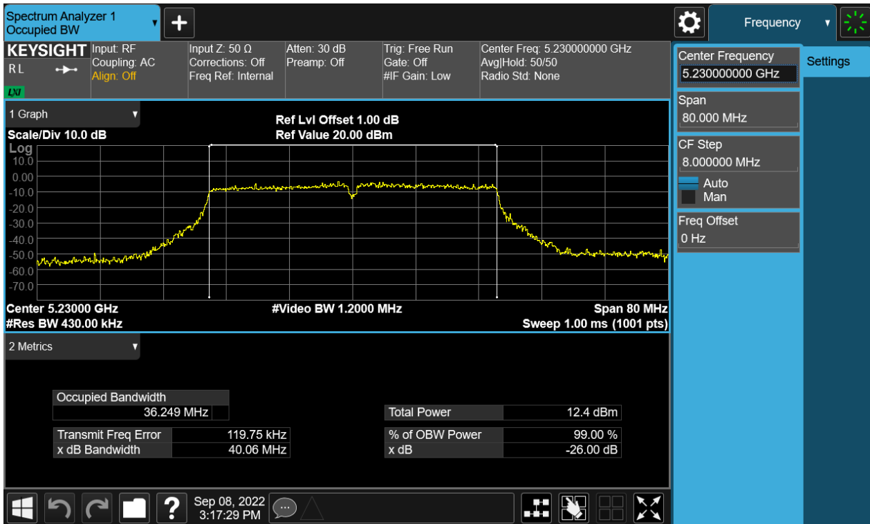
Figure 11: The plots of 26dB Bandwidth and 99% Bandwidth, 802.11n(HT40), 5230MHz
