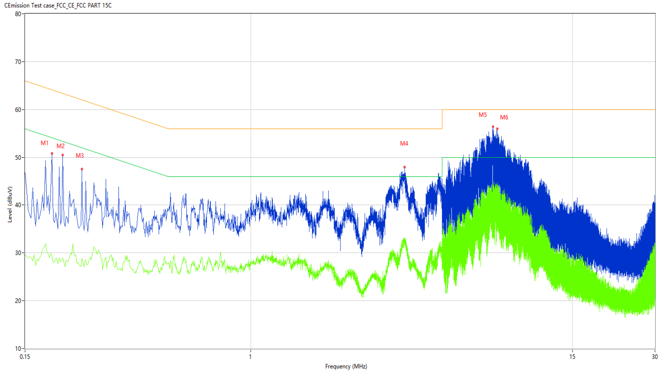
Figure 94: Conducted Emission on AC Mains, N Phase
