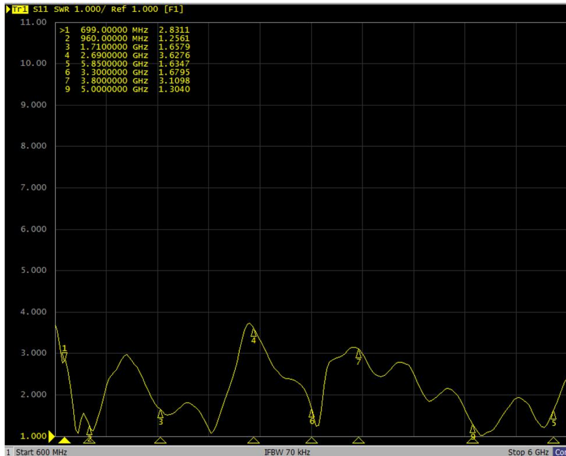
Picture 4 ANT4 antenna VSWR
