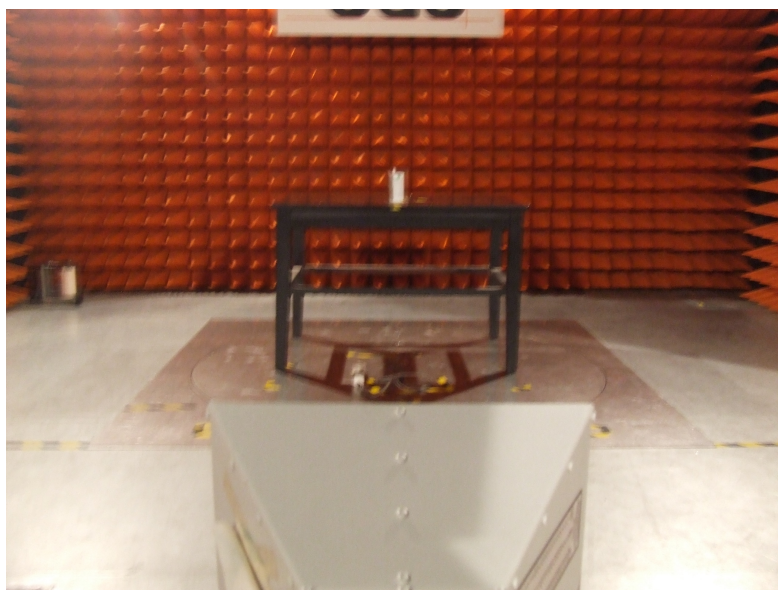
Above 1GHz
